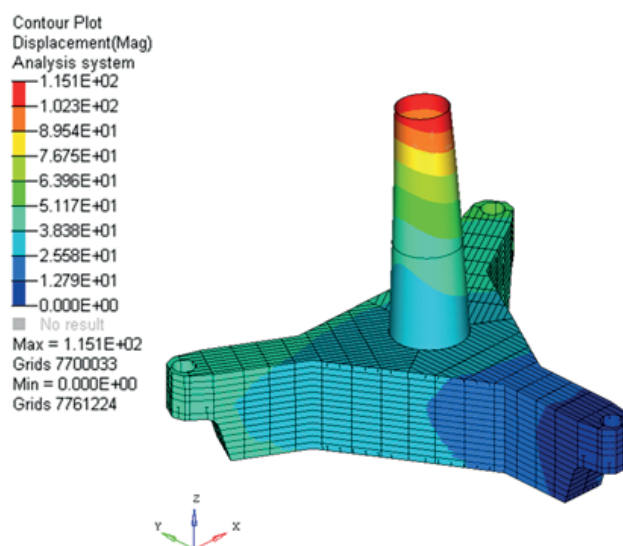
Fig.17. Displacement [mm]
