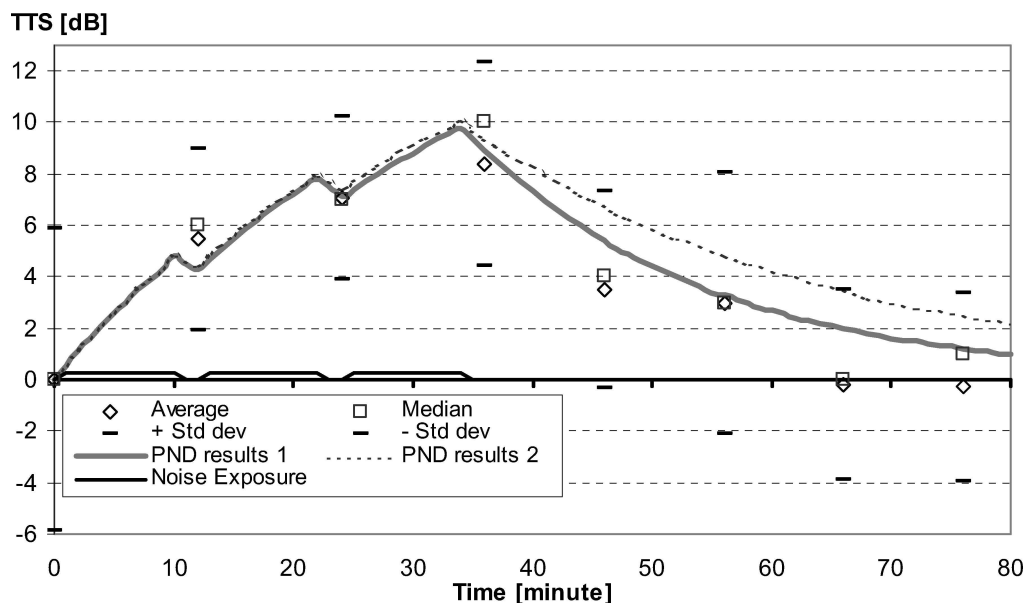
Fig. 2. Measured and simulated TTS changes produced by noise for 4 kHz. The grey and thin black dotted lines reflect the PND results.
