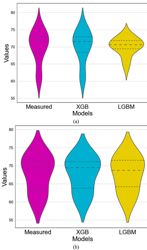
Fig. 8. Violin plots for size reduction model during: (a) Training, (b) Testing.
