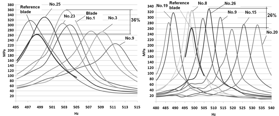
Fig. 5. Maximal stress in blades with 3.6% and 9.5% mistuning for various rotation speeds and for tuned bladed disk (reference blade)
