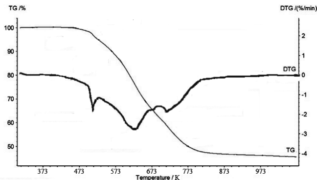
Fig. 6. DTG curve for a mixture, wt parts: pitch – 100; PVC – 3; melamine – 2
