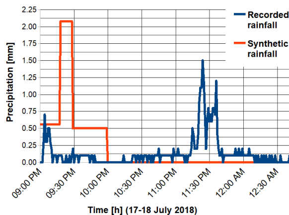
Fig. 2. Synthetic and recorded rainfall used in simulations.
