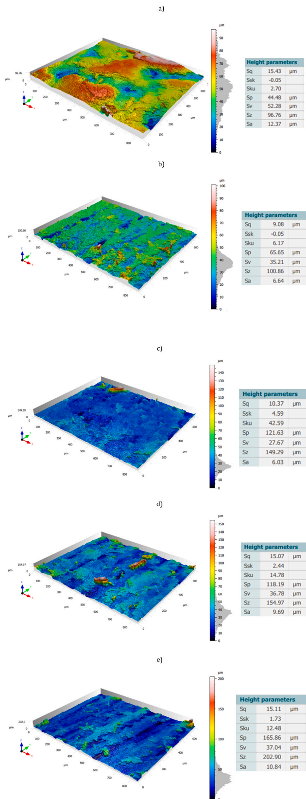
Fig. 11. Exemplary topography of the lapping tools segment #8 on non-contact and highest contact points: a) radius point 55 mm for p-v-, b) radius point 85 mm for p-v-, c) radius point 85 mm for p-v+, d) radius point 85 mm for p+v-, e) radius point 85 mm for p+v+.
