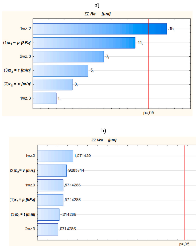
Fig. 18. Pareto plots of the effects of standardized input quantities and their interactions for surface roughness and waviness parameters: a) Ra; b) Wa.
