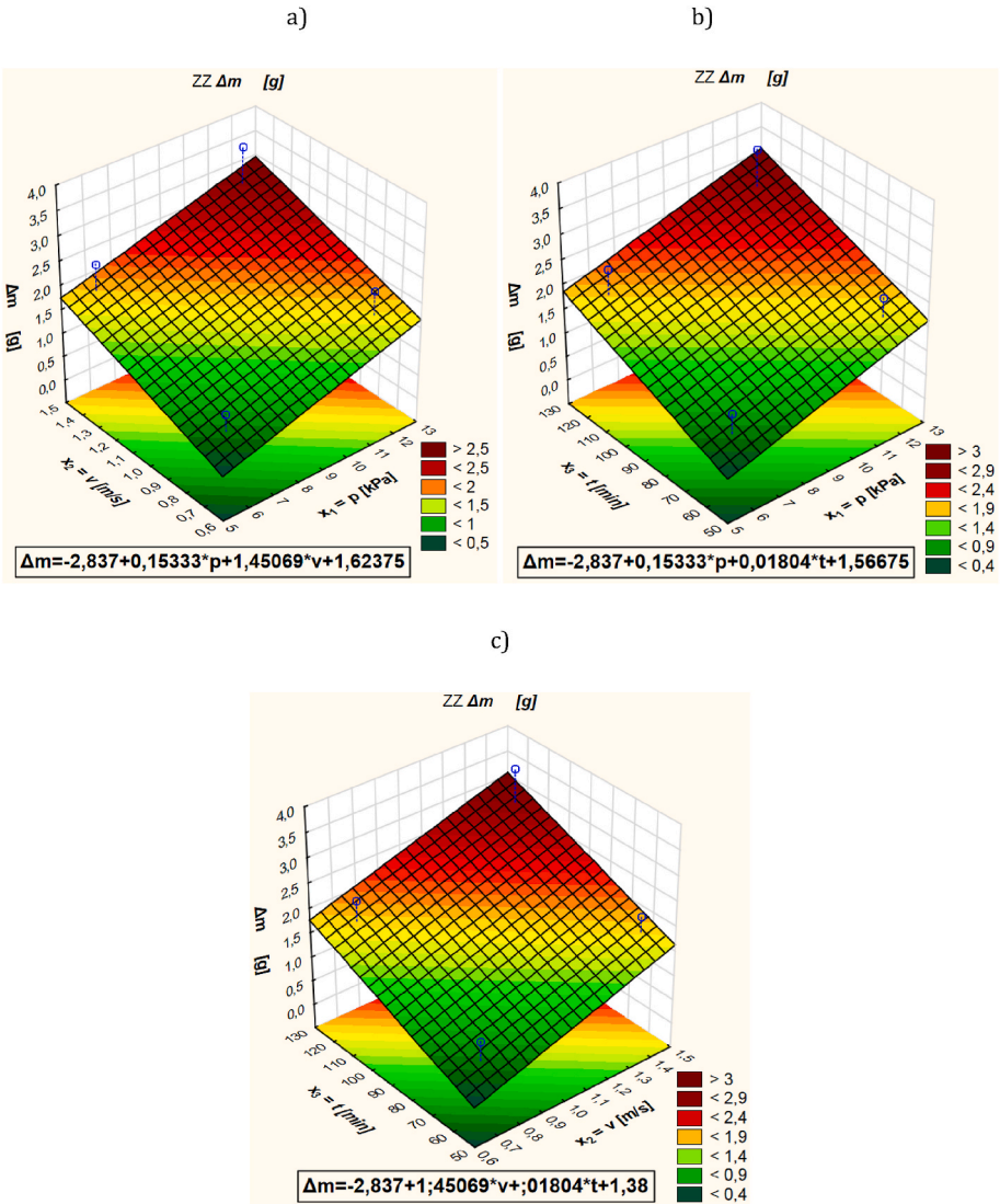
Fig. D.1. Response planes for mass material loss \Delta m : a) constant value of variable x_3 = t = 90 min; b) constant value of the variable x_2 = v = 1.08 m/s; c) constant value of the variable x_1 = p = 9 kPa.
