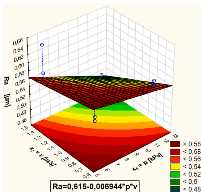
Fig. D.3. Response plane for roughness parameter Ra .
