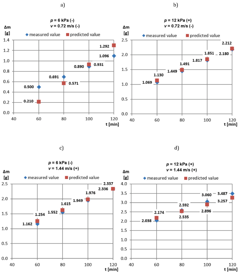
Fig. E.1. Comparison of measured and predicted values for mass material loss \Delta m .
