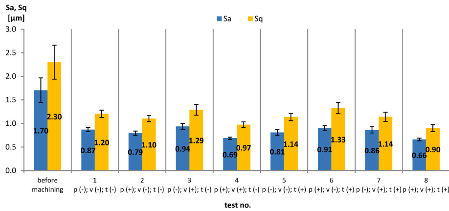
Fig. 15. Average values of Sa and Sq height parameters obtained in particular machining tests; error bars display \pm the standard deviation.
