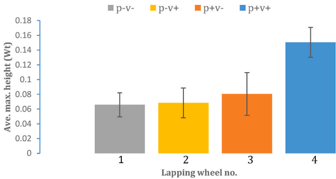
Fig. 10. Average maximum height on the lapping tools wheel.
