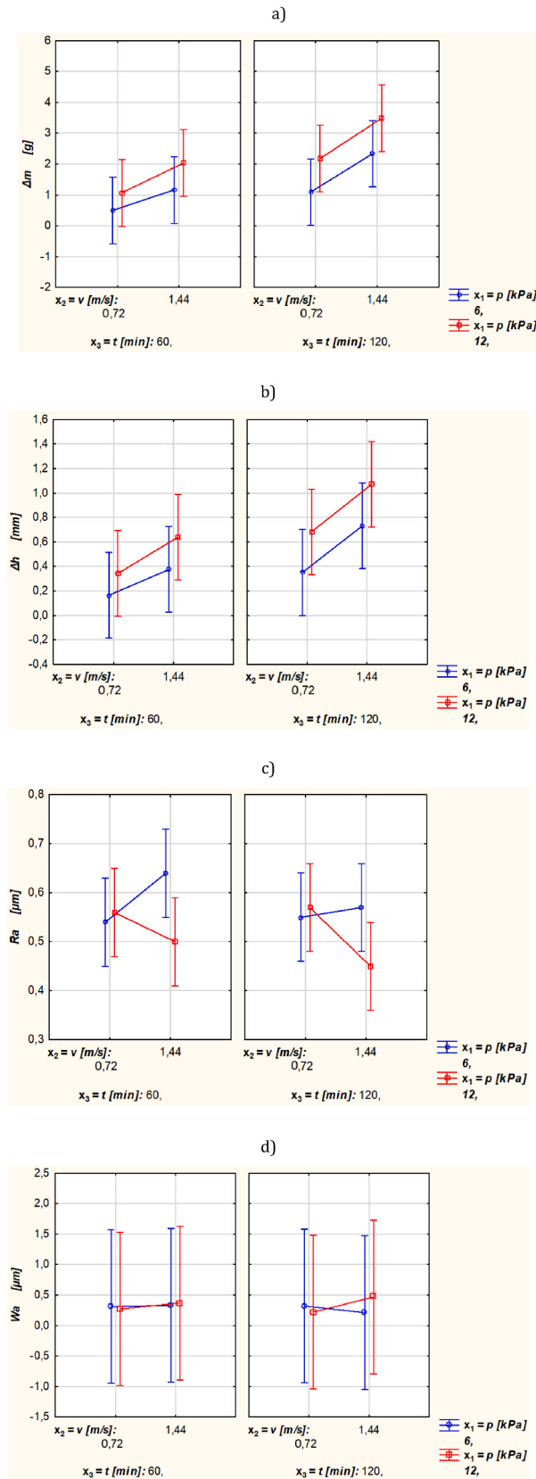
Fig. 14. Interaction diagrams for the analyzed machining results: a) mass material loss \Delta m ; b) linear material loss \Delta h ; c) surface roughness Ra and d) surface waviness Wa ; error bars display \pm the standard deviation.
