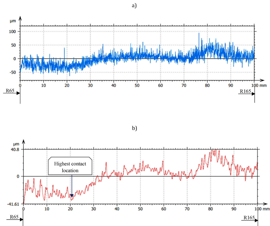
Fig. 7. Exemplary profile of lapping segment #8 after 120 min of machining with p+v-parametric settings: a) raw profile along contact length b) waviness profile along contact length.
