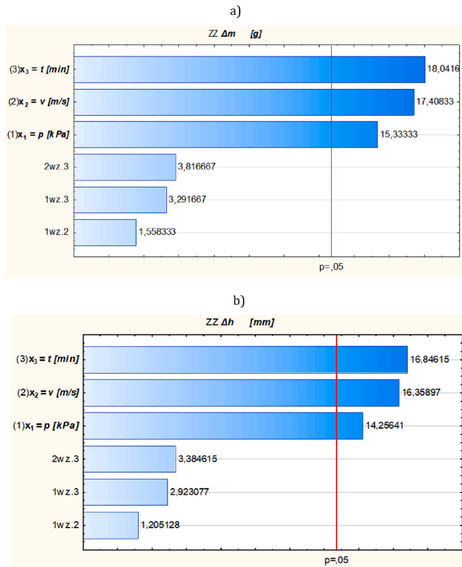
Fig. 17. Pareto plots of the effects of standardized input quantities and their interactions for material loss: a) mass \Delta m ; b) linear \Delta h .
