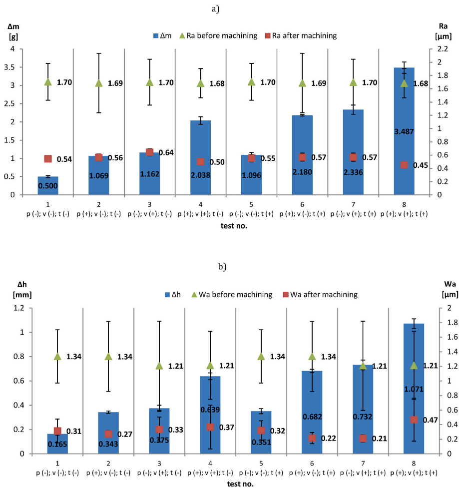
Fig. 13. Technological effects obtained in particular machining tests: a) mass material loss \Delta m and surface roughness Ra ; b) linear material loss \Delta h and surface waviness Wa ; error bars display \pm the standard deviation.
