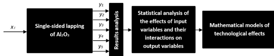
Fig. 2. Scheme of the machining tests of single-sided lapping using different process parameters; characteristics of factors: X – input variables: x_1 – unit pressure p : 6; 12 kPa; x_2 – cutting speed v : 0,72; 1,44 m/s; x_3 – lapping time t : 60; 120 min. Y – output variables: y_1 – linear material removal \Delta h [mm], y_2 – surface roughness (Ra) to less than 5 nm [32], y_3 – mass material loss \Delta m [g], y_4 – 3D surface parameters: S_a , S_q [ \mu\text{m} ] and surface topography [isometric images], y_5 – tool wear [isometric images, 2D profiles and Wt parameters].
