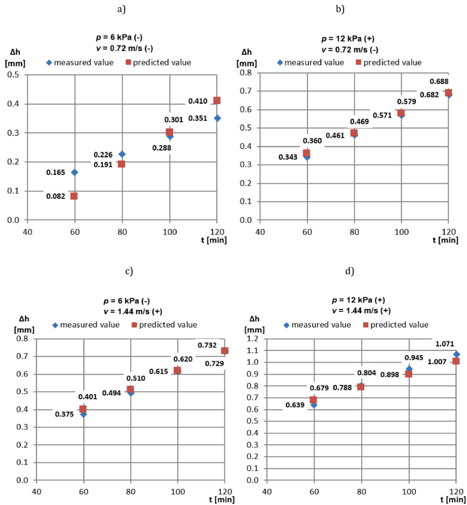
Fig. E.2. Comparison of measured and predicted values for linear material loss \Delta h .
