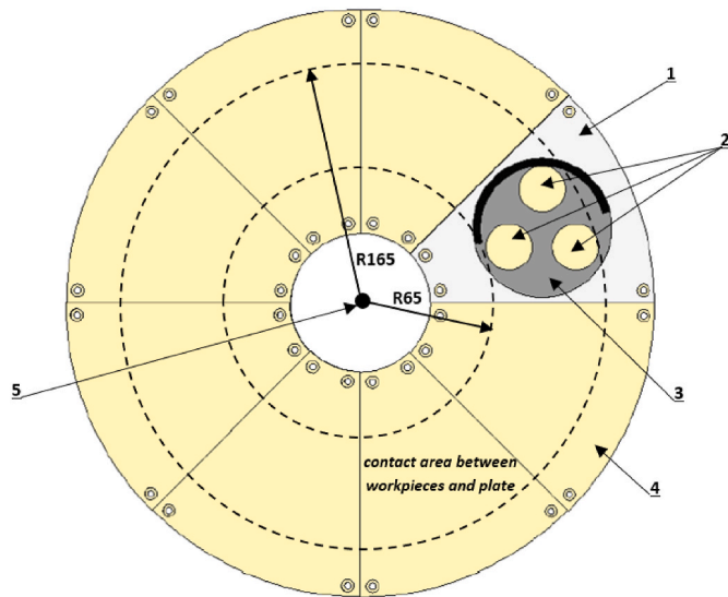
Fig. 4. General kinematic configuration of single-sided lapping station with SLS fabricated abrasive segments; 1 – SLS fabricated single segment, 2 – ceramic workpieces, 3 – workpiece carrier, 4 – lapping plate composed of single segments, 5 – centre of a disc.
