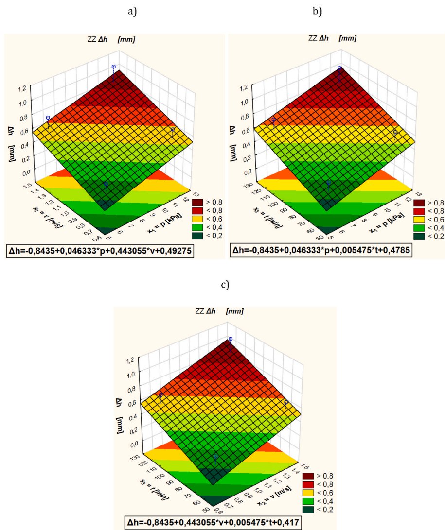
Fig. D.2. Response planes for linear material loss \Delta h : a) constant value of variable x_3 = t = 90 min; b) constant value of the variable x_2 = v = 1.08 m/s; c) constant value of the variable x_1 = p = 9 kPa.
