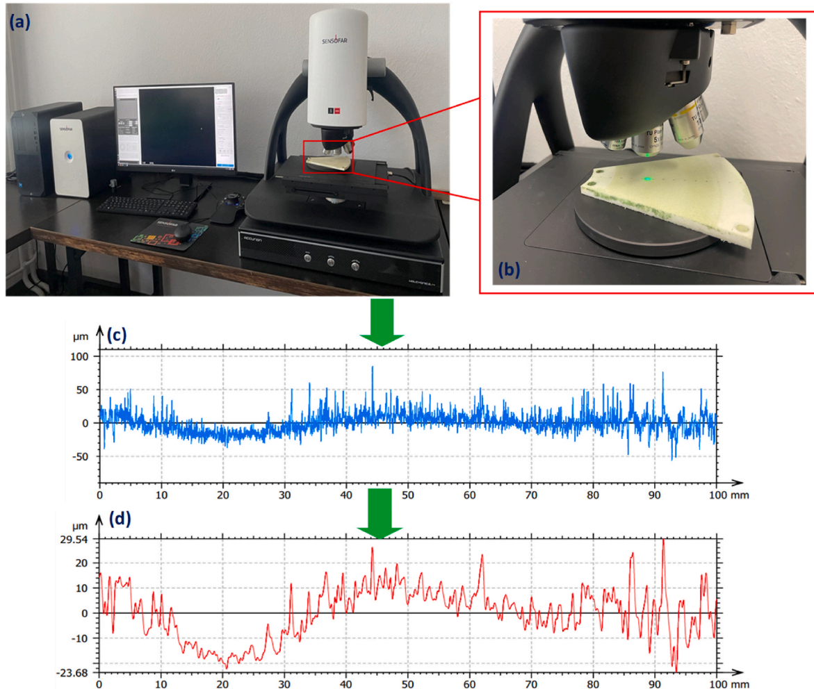
Fig. 3. Measurement station for surface topography assessment: a) Sensofar S neoX 3D optical profilometer with lapping segment on the measuring table, b) detailed views of lapping segment during measurement, c) the radial axis raw profile of contact length, d) the radial axis waviness profile of contact length.
