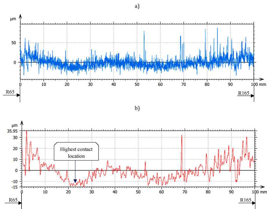
Fig. 5. Exemplary profile of lapping segment #8 after 120 min of machining with p-v- parametric settings: a) raw profile along contact length b) waviness profile along contact length.
