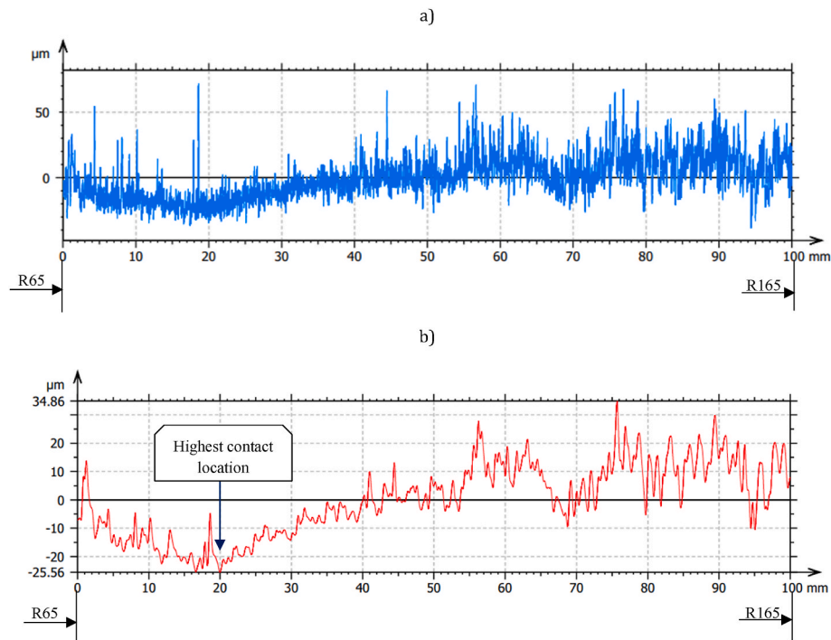
Fig. 6. Exemplary profile of lapping segment #8 after 120 min of machining with p-v+ parametric settings: a) raw profile along contact length b) waviness profile along contact length.
