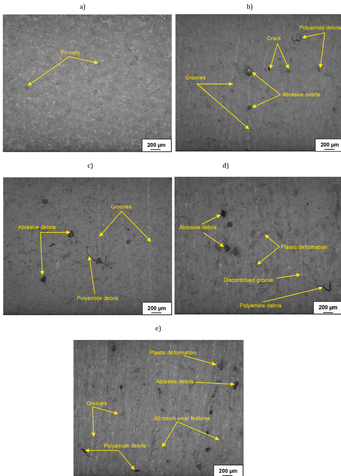
Fig. 12. Surface morphology of an exemplary lapping tools segment #8: a) non-contact region b) radius point 85 mm for p-v-, c) radius point 85 mm for p-v+, d) radius point 85 mm for p+v-, e) radius point 85 mm for p+v+.
