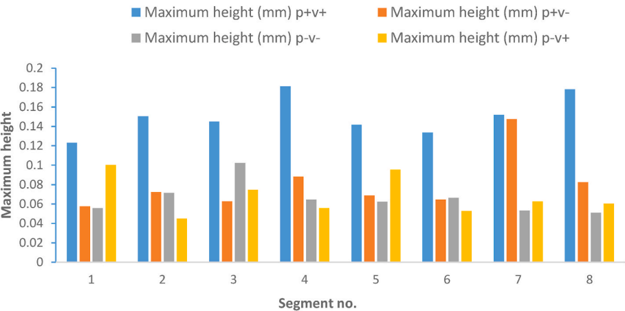
Fig. 9. Parametric maximum height values of the lapping tools segments.
