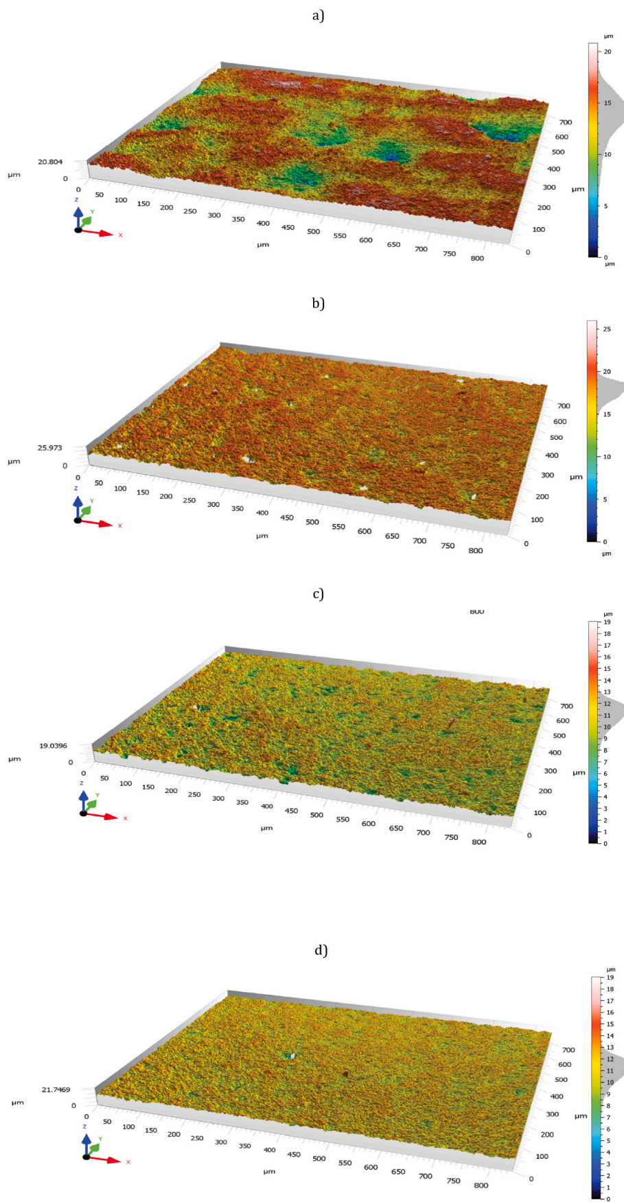
Fig. 16. Selected surface topographies of ceramic workpieces: a) before machining; b) after test no. 6 ( p = 12 \text{ kPa} , v = 0.72 \text{ m/s} , t = 120 \text{ min} ); c) after test no. 7 ( p = 6 \text{ kPa} , v = 1.44 \text{ m/s} , t = 120 \text{ min} ) and d) after test no. 8 ( p = 12 \text{ kPa} , v = 1.44 \text{ m/s} , t = 120 \text{ min} ).
