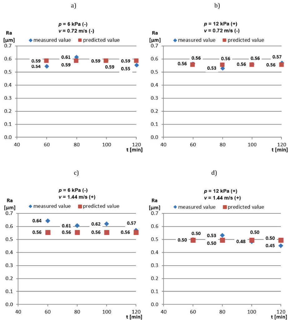
Fig. E.3. Comparison of measured and predicted values for roughness parameter R_a .
