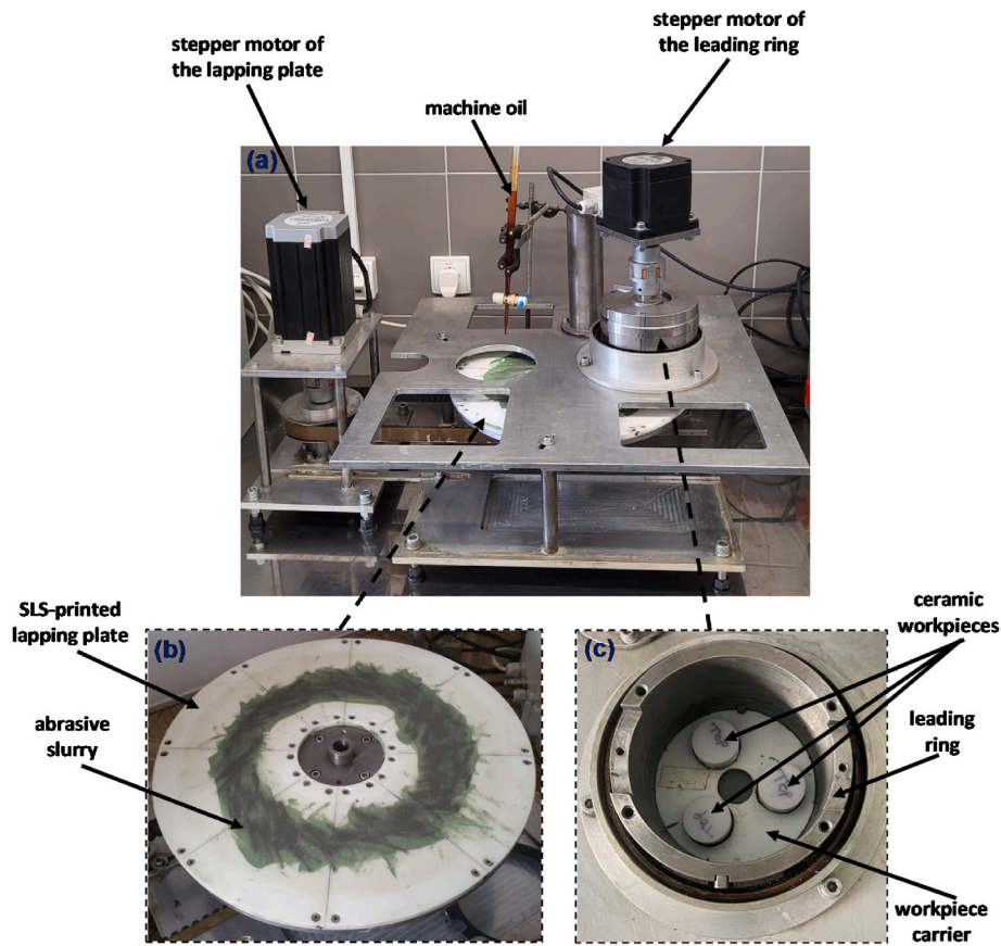
Fig. 1. Experimental setup: a) single sided lapping station, b) detailed view of SLS-printed polyamide lapping plate with abrasive slurry, c) detailed view of \text{Al}_2\text{O}_3 ceramic samples inside leading ring.
