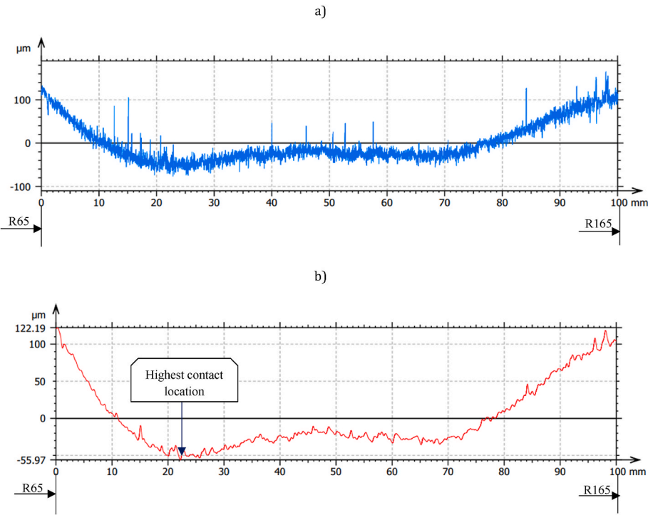
Fig. 8. Exemplary profile of lapping segment #8 after 840 min of machining with p+v+ parametric settings: a) raw profile along contact length b) waviness profile along contact length.
