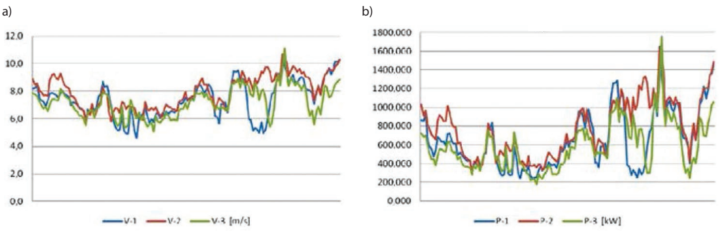
Fig. 1. Wind speeds and wind turbine output powers in a vast wind farm (for the period of one day)
