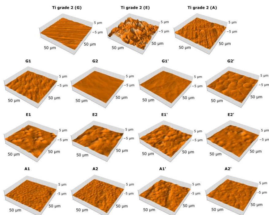
Figure 4. Surface topographies obtained by atomic force microscopy of the investigated samples.
