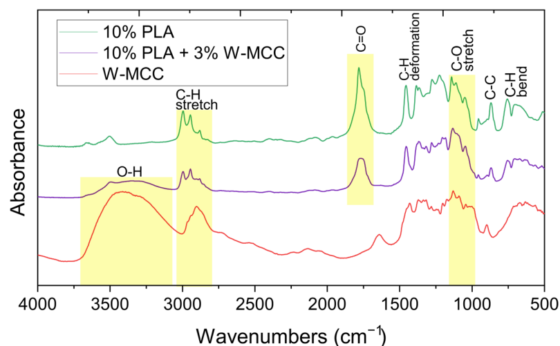
Figure 5. FT-IR spectra of 10% PLA, 10% PLA+3% W-MCC, and W-MCC.
