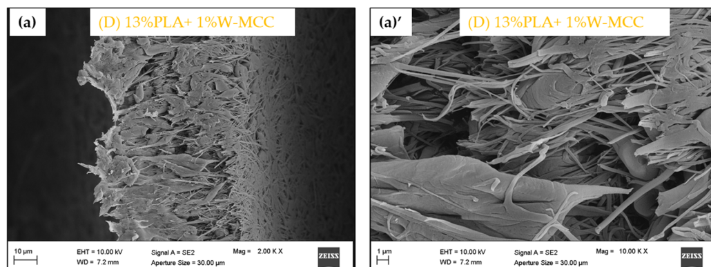
Figure 3. FESEM images ((a), (a')) of the cross section of (D) 13% PLA+1% W-MCC.
