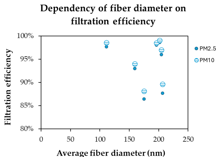
Figure 8. Relationship between the fiber diameter and filtration efficiency of PLA-based filters.
