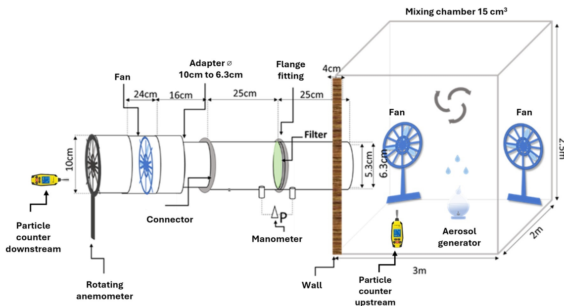
Figure 12. Schematic diagram of the testing room (figure not to scale).
