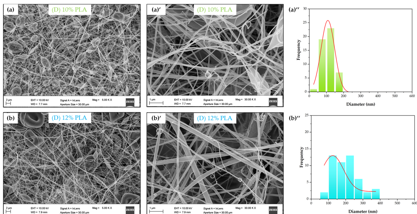
Figure 4. Morphological analysis of fabricated filters: FESEM images ((a),(b), (a)',(b')) and diameter fiber distributions ((a''),(b'')) of electrospun PLA fibers.
