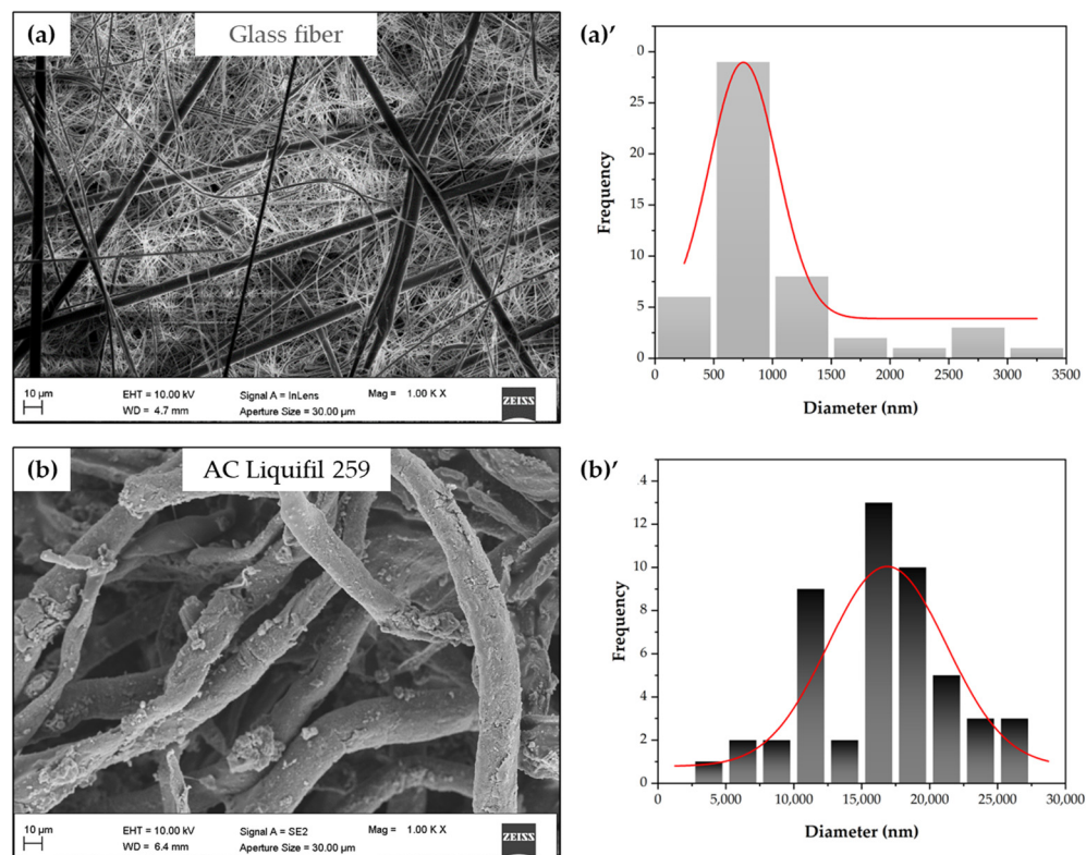
Figure 1. Morphological analysis of commercial filters: FESEM images of glass fiber (a), and AC Liquifil 259 (b), and diameter fiber distributions ((a'), (b')) of commercial filters.
