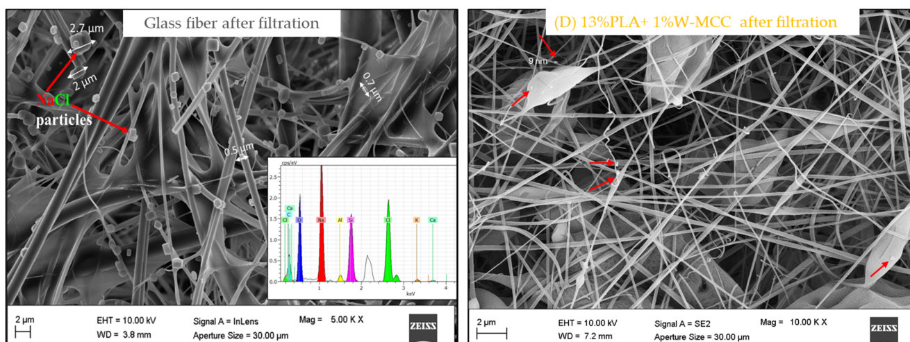
Figure 9. FESEM images of glass fiber and 13% PLA+1% W-MCC after the filtration test. Filtered particles are indicated with red arrows.
