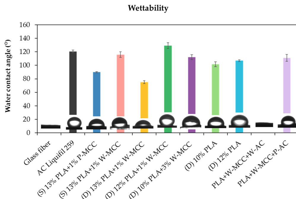
Figure 11. Comparison of the contact angle values for PLA and PL/MCC fibers.
