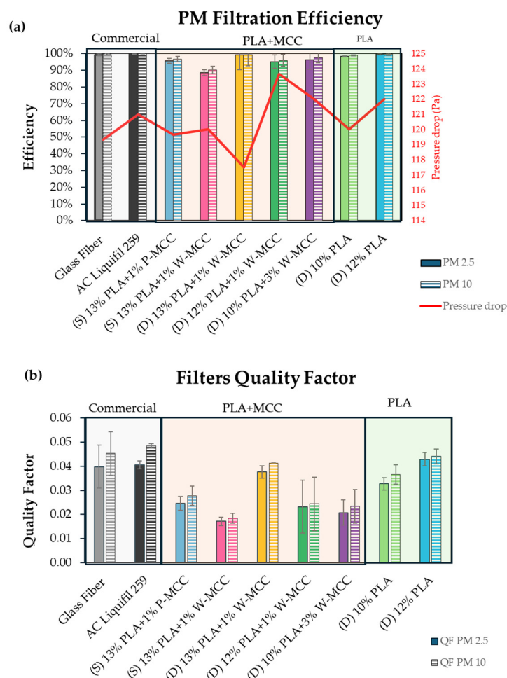
Figure 7. (a) Filtration efficiency results and (b) quality factors.
