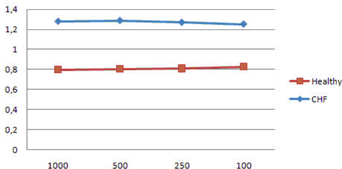
Fig. 2. Values of \text{FuzzyEn}(2,0.2,N) for decreasing N .
