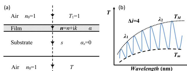
Fig. 13. For a light absorbing thin film supported on a thick, finite, transparent substrate a) the interference effects will give rise to the transmitted signal producing interference fringes, confined by two envelopes T_M and T_m b). \lambda_1 , \lambda_2 , and \Delta i according to the text [102].
