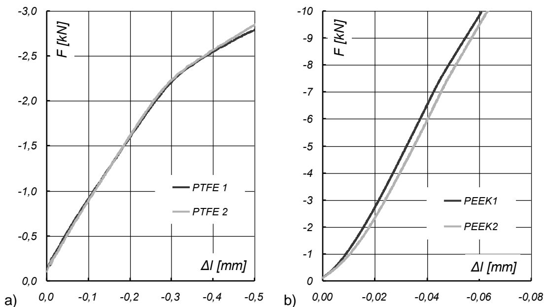
Figure 5. Comparison of the compression results obtained for both samples at 120 C°; a) PTFE lined sample (3 rd repetition), b) PEEK lined sample (4 th repetition).
