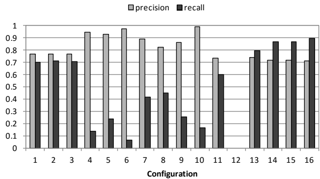
Figure 3. Precision and recall metrics for person No. 1, conditions C1
