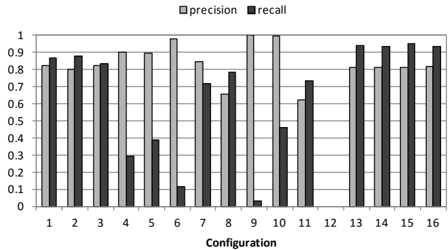
Figure 4. Precision and recall metrics for person No. 1, conditions C2
