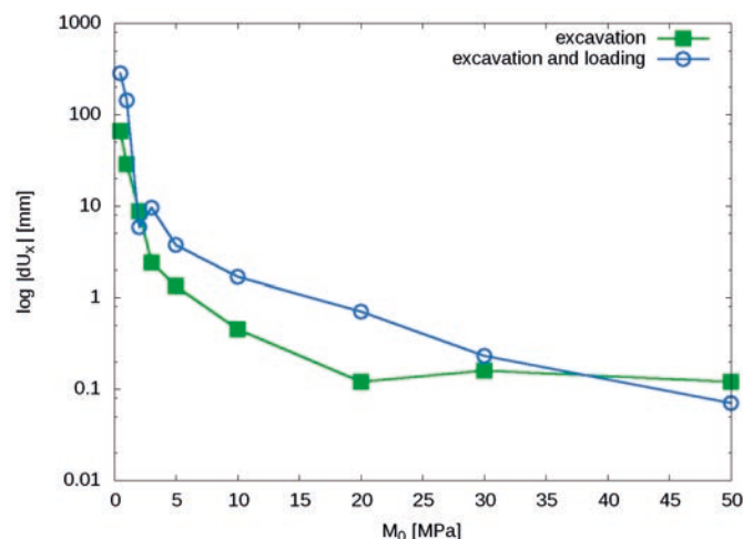
Figure 2. Upper-bound case (pipe with no stiffness) horizontal differential displacements |U_x^A - U_x^B| plotted against subsoil oedometric modulus
