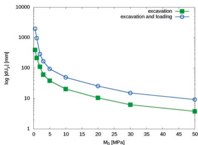
Figure 3. Upper-bound case (pipe with no stiffness) vertical differential displacements |U_y^A - U_y^B| plotted against subsoil oedometric modulus
