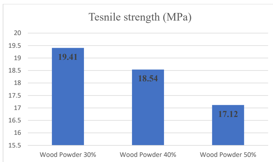
Figure 6. Tensile strength comparison according to a different amount of wood powder and 0% nanoclay.
