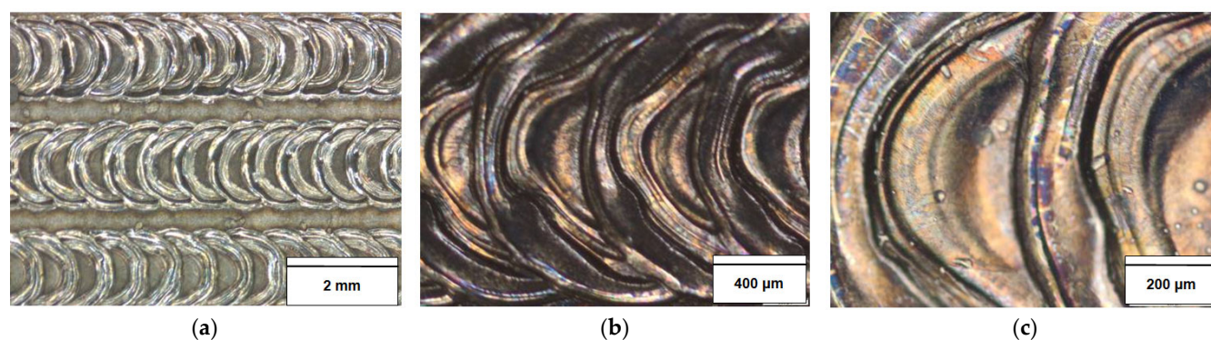
Figure 10. Etched and blackened AISI 316L surface subjected to laser texturing of 2500 W laser beam power with pulse focus of 0.5 mm and frequency of 3 Hz: (a) 10× magnification by ZEISS; (b) 50× magnification by Olympus; and (c) 100× magnification by Olympus.
