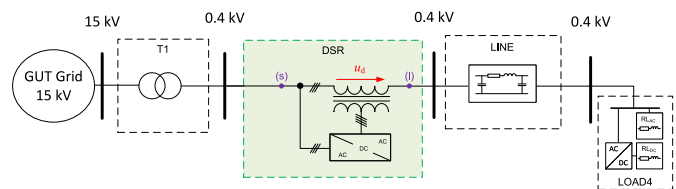
Fig. 5. Test system topology - case 1.
