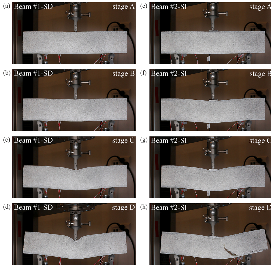
Fig. 6. Deformations of beams in selected stages during bending: (a)÷(d) Beam #1-SD, (e)÷(h) Beam #2-SI.
