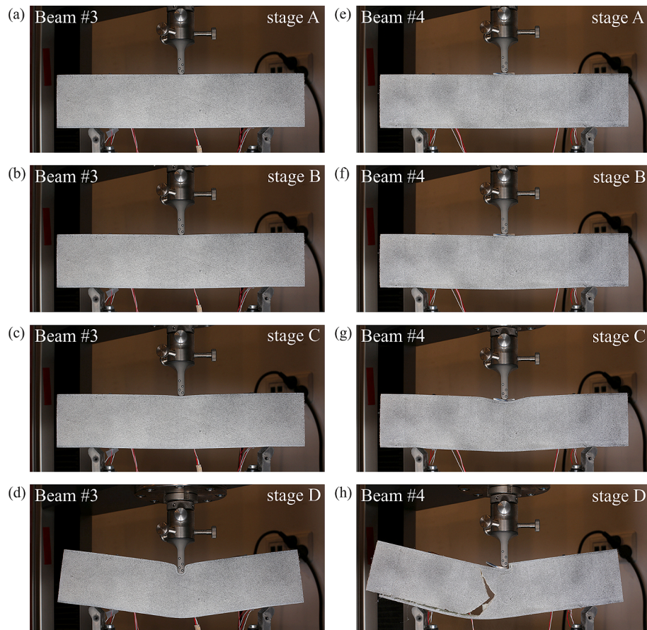
Fig. 9. Deformations of beams in selected stages during bending: (a)–(d) Beam #3-HD, (e)–(h) Beam #4-HI.
