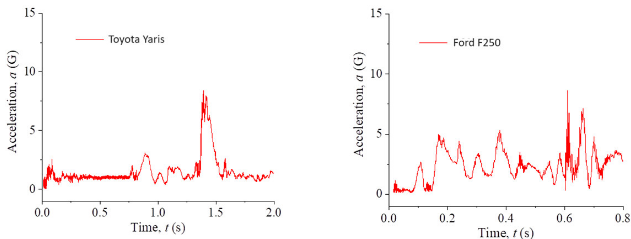
Figure 23. Head resultant accelerations from the 25^\circ impacts at the nearest corner of dual-unit Type I CM behind a curb (D4).
