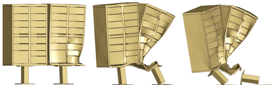
Figure 17. Sequential deformation of the dual-unit Type IV CM impacted by Toyota Yaris at 25° and at the nearest corner on a flat road. Time steps shown are 20, 80, and 120 ms.
