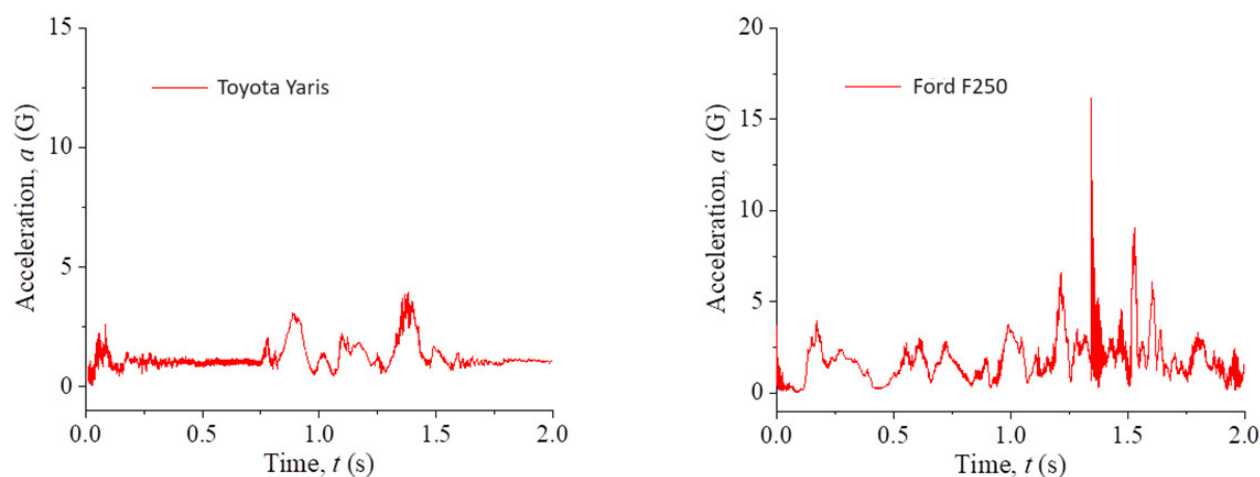
Figure 24. Head resultant accelerations from the 25^\circ impacts at midpoint of dual-unit Type I CM behind a curb (D5).
