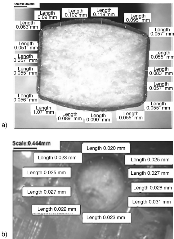
Figure 3. Cross-section area with film thickness measured on minitabets (a) and pellets (b).
