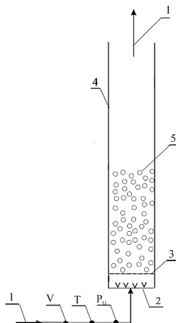
Figure 2. Experimental set-up for determination of minimum fluidization velocity (1 – air stream, 2 – fluid distributor, 3 – metal mesh, 4 – column, 5 – solid particles bed, P G – manometer, T – thermometer, V – rotameter).
