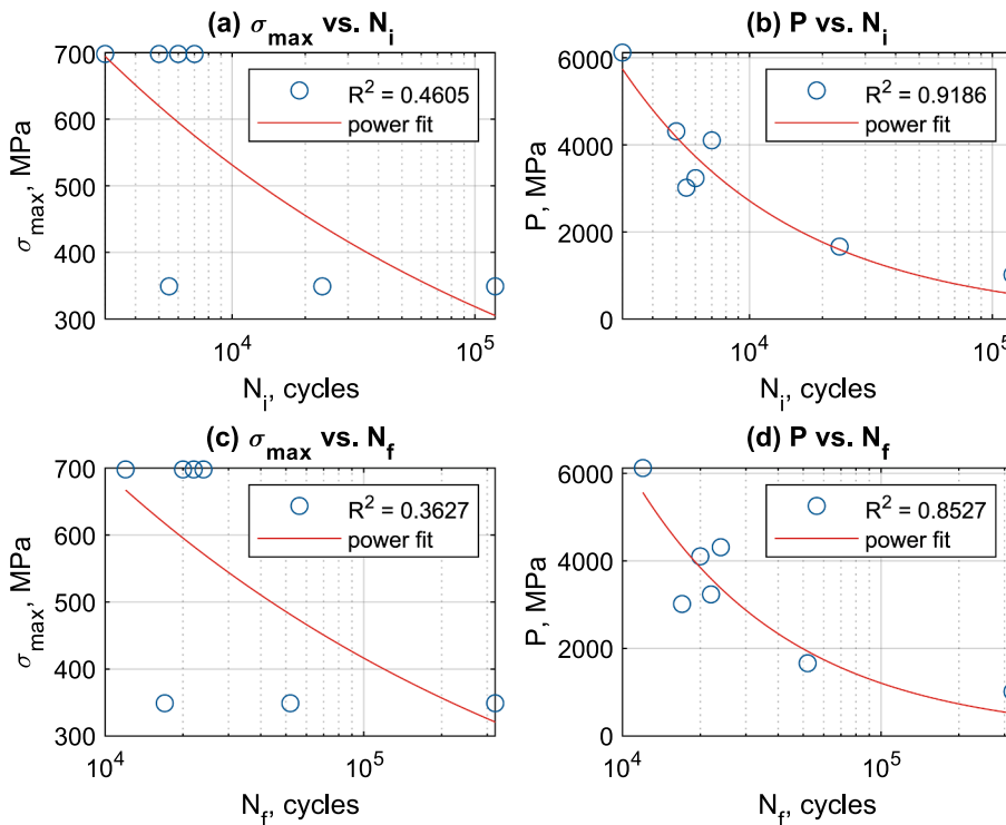
Fig. 20. Power fit relationship between: (a) maximum bending stress \sigma_{max} versus N_i ; (b) topographic stress factor P versus N_i ; (c) maximum bending stress \sigma_{max} versus N_f and (d) topographic stress factor P versus N_f .
