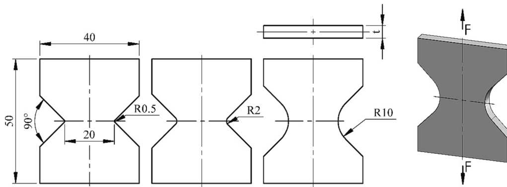
Fig. 2. Notched specimens [31].
