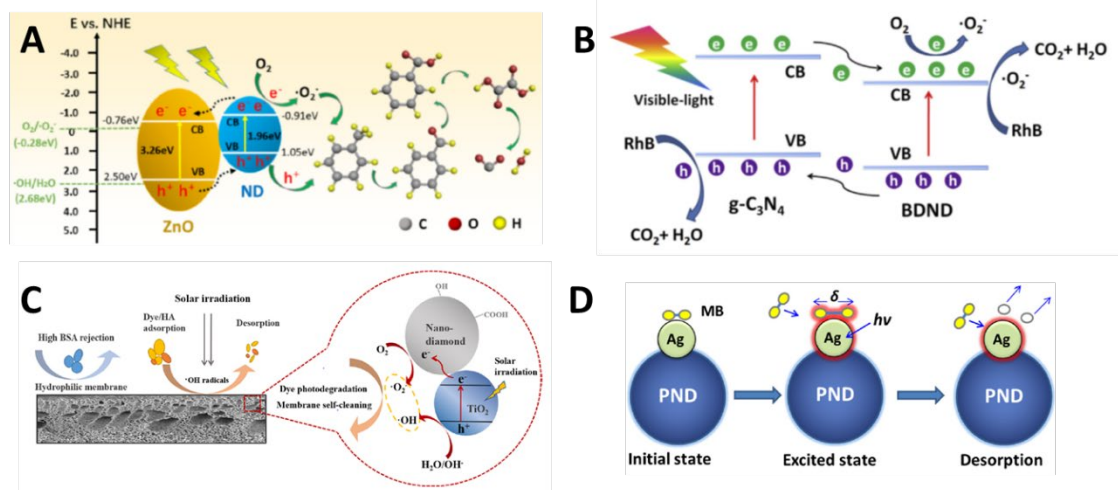
Figure 9. (A) Mechanism for photocatalytic degradation of toluene using nanodiamond - ZnO complexes. Reproduced with permission from Ref. [57]. Copyright 2019, Elsevier. (B) Enhanced photocatalytic degradation of rhodamine B at boron-doped nanodiamond at g-C 3 N 4 nanosheets. Reproduced with permission from Ref. [15]. Copyright 2019, Elsevier. (C) The self-cleaning effect at complex photocatalytic membrane PVDF-carboxylated nanodiamond/TiO 2 . Reproduced with permission from Ref. [58]. Copyright 2015, American Chemical Society, (D) Process of plasmon-induced photodegradation of methylene blue using silver deposited at pyridine modified nanodiamonds. Reproduced with permission from Ref. [56]. Copyright 2015, Elsevier.
