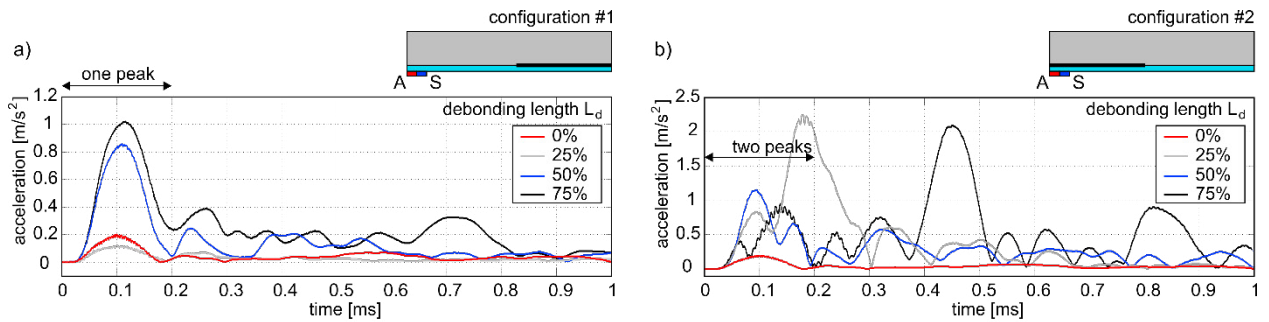
Fig. 5. Envelopes of signals registered for beams with various debonding length: (a) configuration #1; (b) configuration #2.
