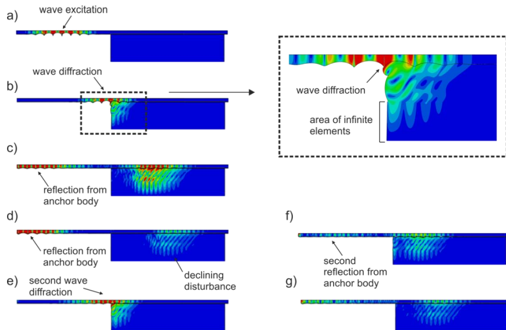
Figure 4.14. Snapshots of propagating waves (magnitude of acceleration) in ground anchor with non-reflecting boundary conditions at selected time instants a) t = 0.13 ms ; b) t = 0.21 ms ; c) t = 0.32 ms ; d) t = 0.37 ms ; e) t = 0.50 ms ; f) t = 0.58 ms ; g) t = 0.62 ms
