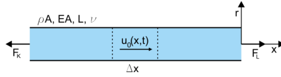
Figure 2.2 Segment of a rod with end loads
