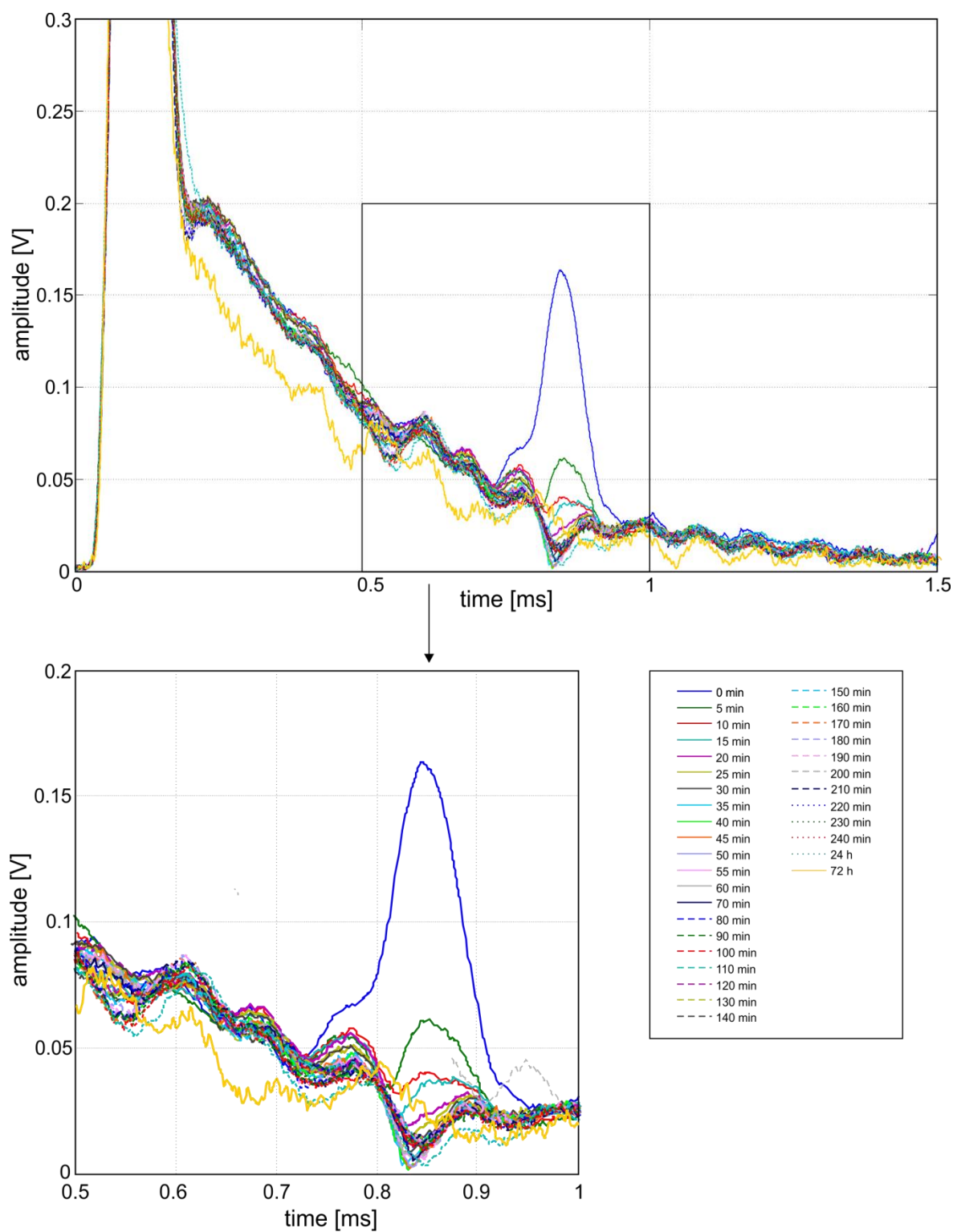
Figure 7.13 Envelopes of signals registered at the end of the anchor performed in the ground during hardening process (excitation frequency: 60 kHz)
