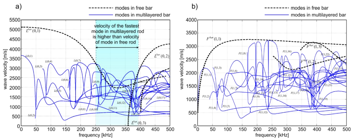
Figure 6.2. Group velocity dispersion curves of 1 cm diameter steel bar ( E = 207 GPa, \nu = 0.3 , \rho = 7894 kg/m 3 ) embedded in mortar with thickness of 17.5 mm ( E = 23.68 GPa, \nu = 0.2 , \rho = 2067 kg/m 3 ) formed in PVC pipe with thickness of 2.5 mm ( E = 1.5 GPa, \nu = 0.4 , \rho = 900 kg/m 3 ): a) longitudinal modes, b) flexural modes
