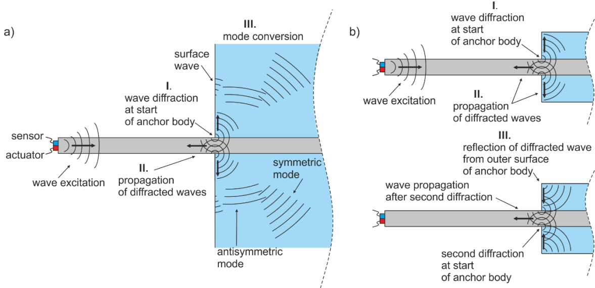
Figure 4.6. Wave diffraction at start of anchor body: a) anchor body thickness much smaller than the excited wavelength; b) anchor body thickness comparable with the excited wavelength
