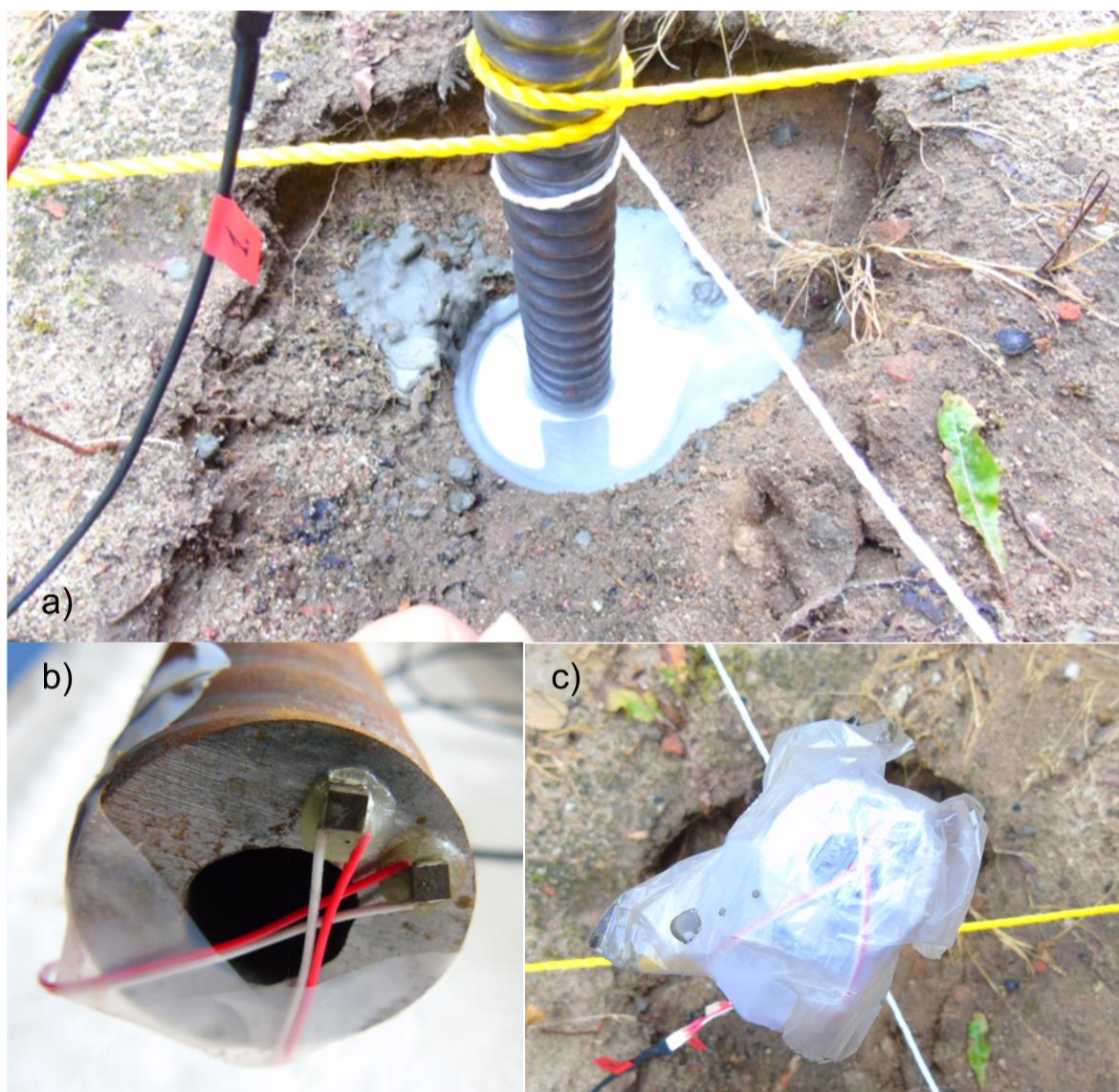
Figure 7.12 Small-scale anchor model performed in the ground: a) self-drilling bar placed in liquid mortar, b) sensor and actuator located at the end of the bar before placing in the ground and c) transducers protected against unfavorable environmental conditions
