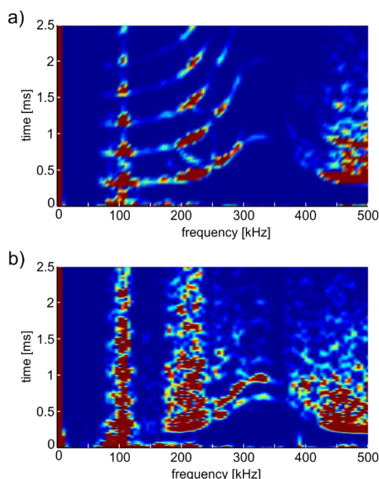
Figure 6.16. Spectrogram of ultrasonic signals registered in the free bar: a) intact bar, b) bar with crack
