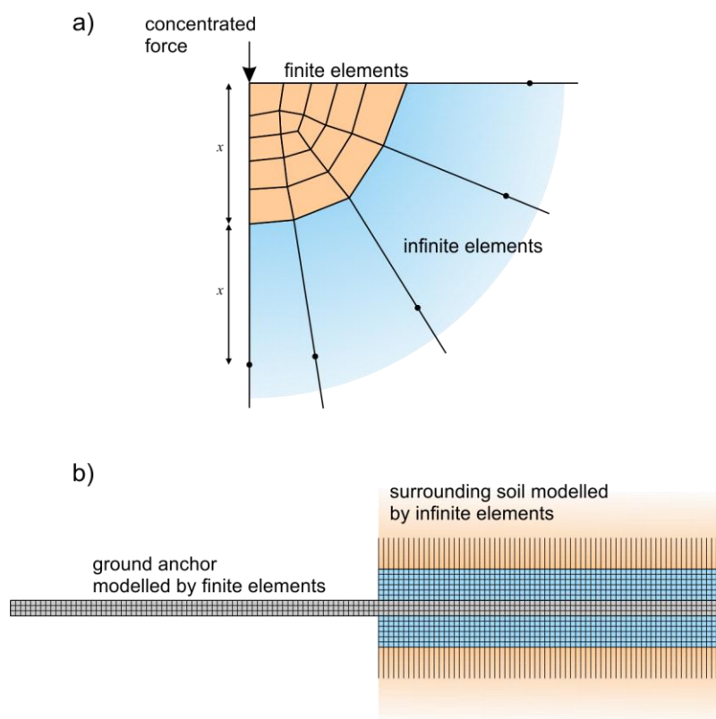
Figure 3.4 Application examples of infinite elements: a) point load on elastic half space [1] and b) ground anchor surrounded by the soil
