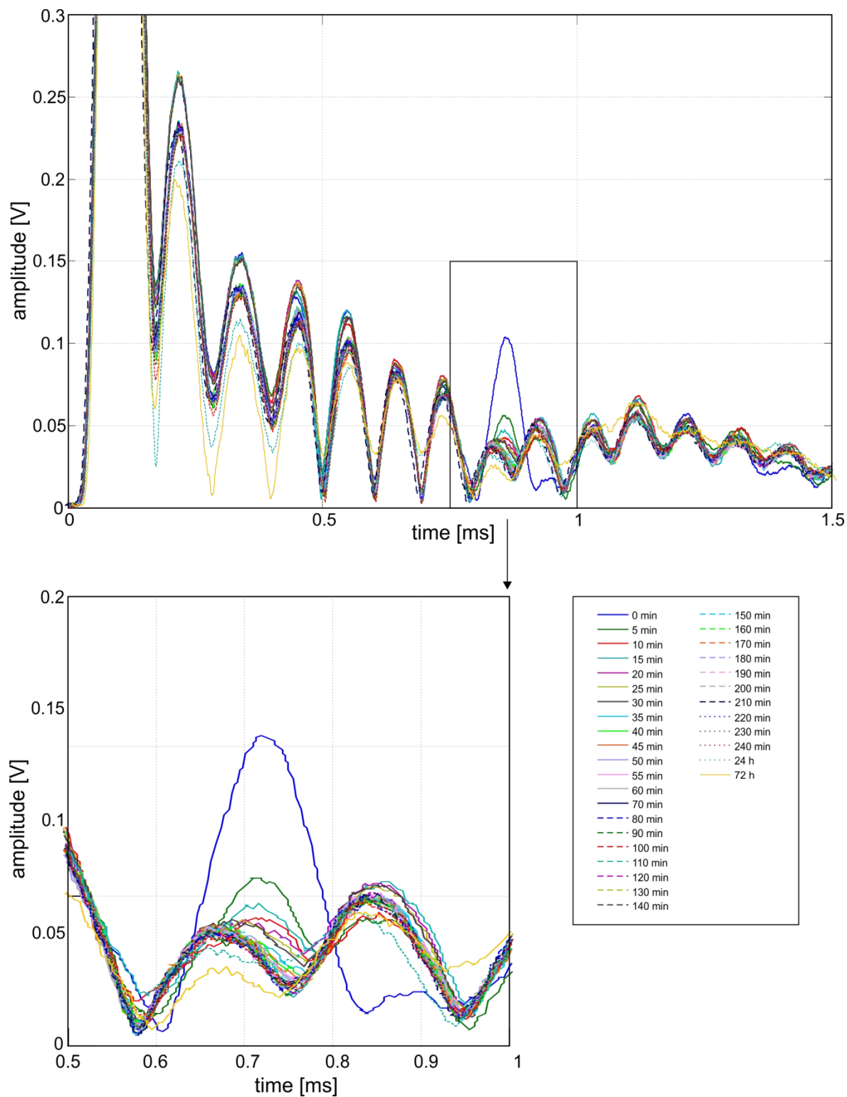
Figure 7.14 Envelopes of signals registered at the end of the anchor performed in the ground during hardening process (excitation frequency: 70 kHz)
