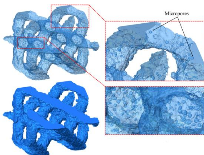
Fig. 11. Micropores in geometric models obtained on the basis of microtomographic images on the example of a diamond structure with a relative density of 27%.
