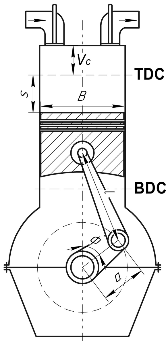
Fig. 4. Schematic diagram of the crankshaft mechanism
