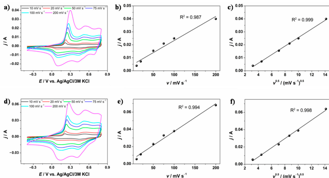
Figure 6. Cyclic voltammetry curves registered at different scan rates for (a) GF/PANI and (d) GF/PANI/PEDOT:PSS; plots of j = f(v) and j = f(v^{1/2}) at E = 0.3 V for GF/PANI (b,c) and GF/PANI/PEDOT:PSS (e,f).
