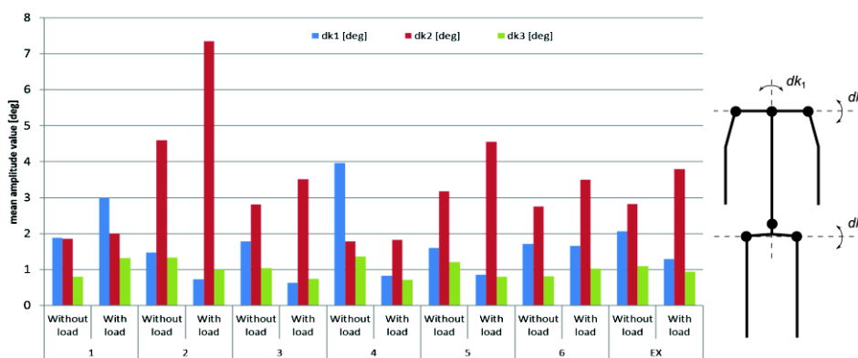
Figure 4. Motion capture results (mean amplitude) in a front view: longitudinal axis deviation ( dk_1 ), shoulder girdle ( dk_2 ) and pelvis tilt ( dk_3 ); during gait without and with load for each of six volunteers
