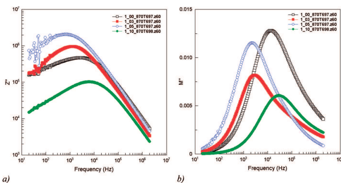
Fig. 3. Influence of bismuth content on spectroscopic plots of Z''(\nu) (a) and M''(\nu) (b) for BiNbO 4 ceramics at T \approx 425^\circ\text{C}
