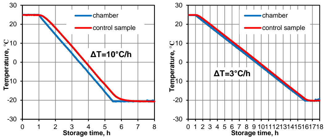
Fig. 5. Temperature charts during conditioning process.
