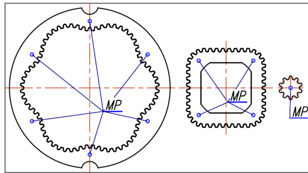
Figure 11. Points MP for measuring the height H_E of the curvature, the height H_R of the rotor and the height H_S of the satellite.
