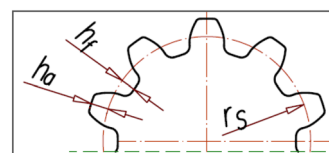
Figure 3. Basic parameters of the satellite: h_a —addendum, h_f —dedendum, r_s —the reference radius.
