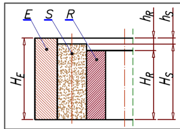
Figure 10. The height H_E of the curvature, the axial clearance h_S of the satellite, the axial clearance h_R of the rotor.
