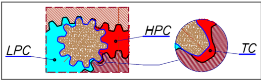
Figure 38. Unfavourable position of the satellite in relation to the rotor—large intertoothed and tip clearances of the interacting teeth.
