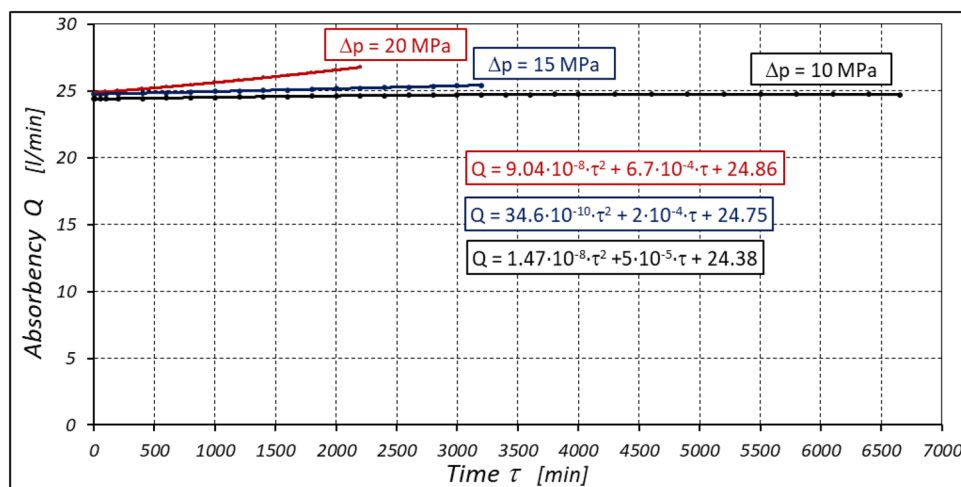
Figure 30. Characteristics of the motor absorptency Q as a function of time \tau for different fixed pressure drop \Delta p in the motor.
