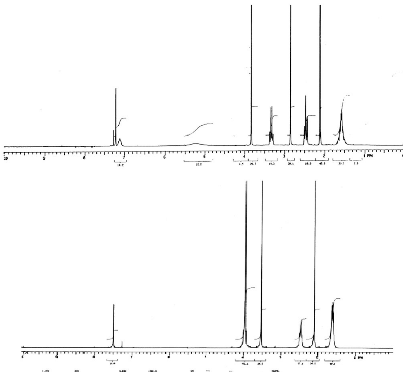
Fig. 8 ^1\text{H} NMR (200 MHz, \text{CDCl}_3 ) of pentoxifylline and its degradation product
