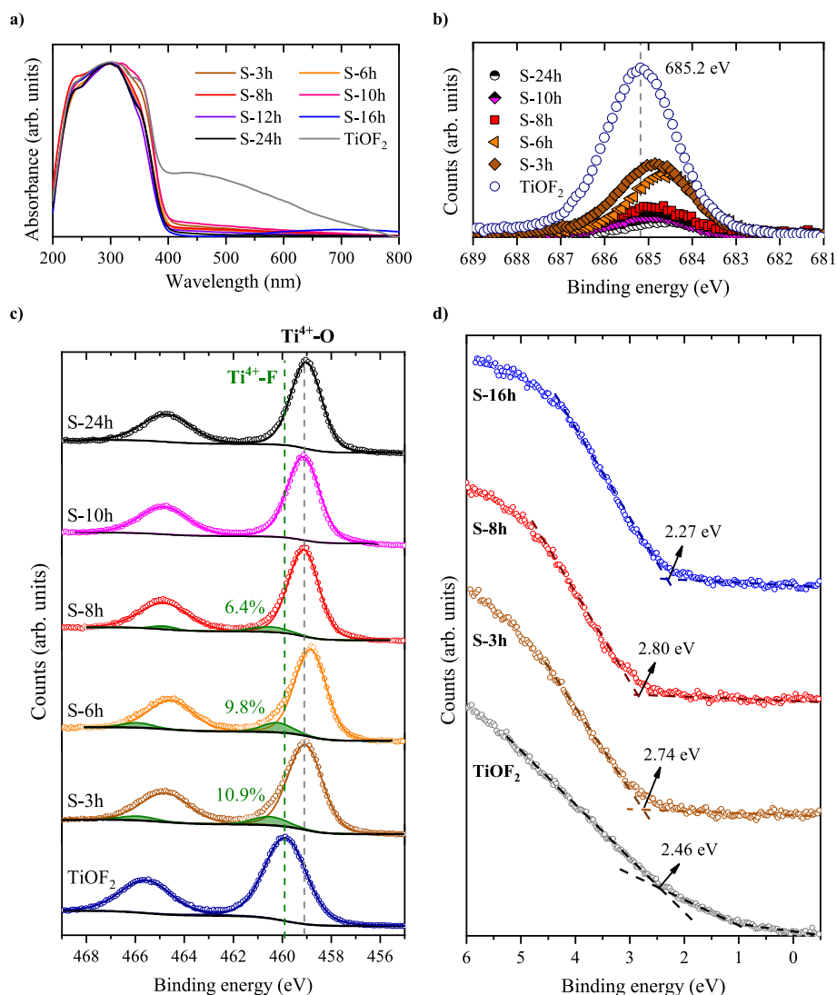
Fig. 3. a) DR/UV-vis absorption spectra of the photocatalysts, b) F1s and c) Ti2p orbital XPS spectra recorded on selected samples from the \text{TiO}_2/\text{TiOF}_2 series, d) VB-XPS spectra of selected photocatalysts.
