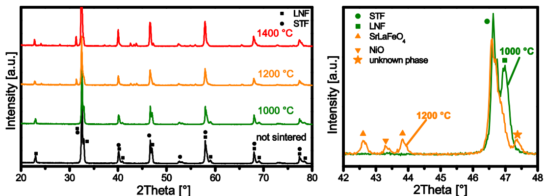
Fig. 2. XRD patterns of the STF-LNF mixture.
