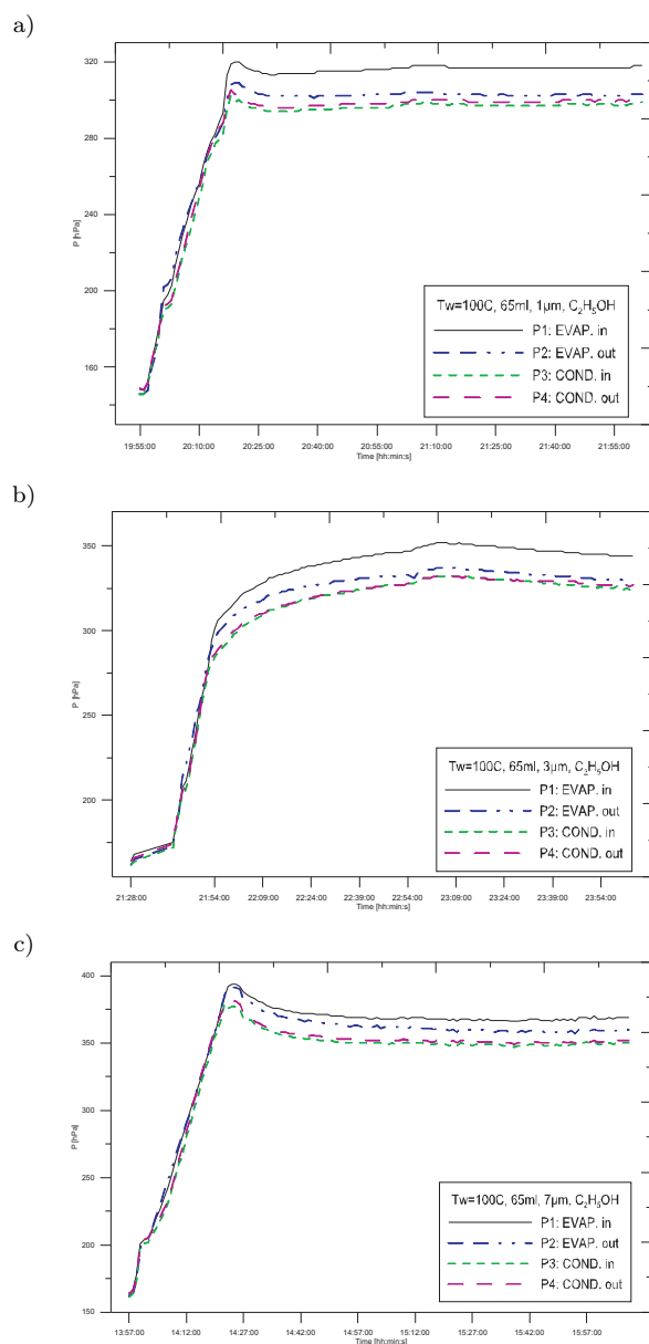
Figure 12: Pressure distribution in function of time in four specific nodes of installation. Working fluid-ethanol, T_w = 100^\circ\text{C} , filling volume 65 ml, pore size a) d_p = 1 \mu\text{m} , b) d_p = 3 \mu\text{m} , c) d_p = 7 \mu\text{m} .
