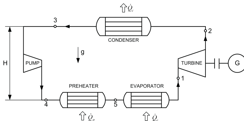
Figure 2: Structural scheme of the ORC cycle.
