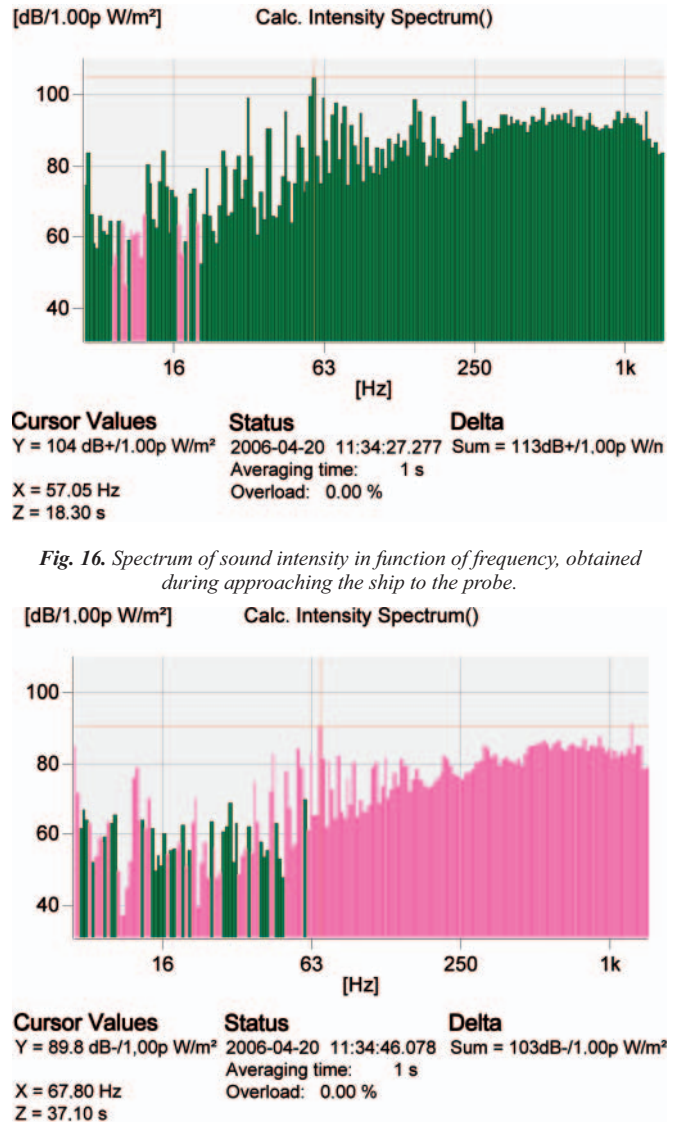
Fig. 17. The spectrum of sound intensity in function of frequency, obtained during departing the ship from above the probe
