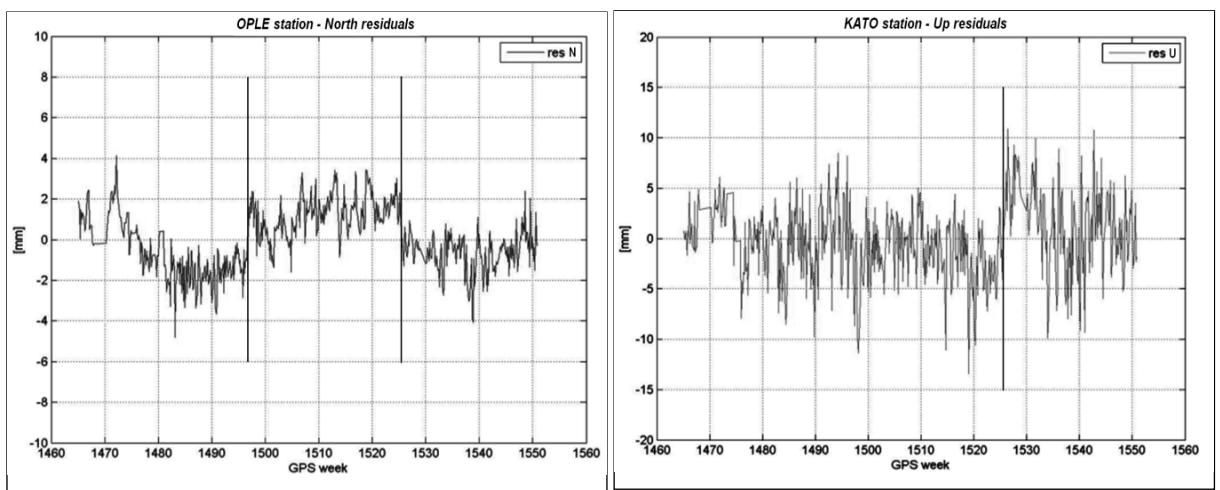
Fig. 16 Examples of time series in which discontinuities can be observed; on the left North residuals (OPLÉ), on the right Up residuals (KATO).
