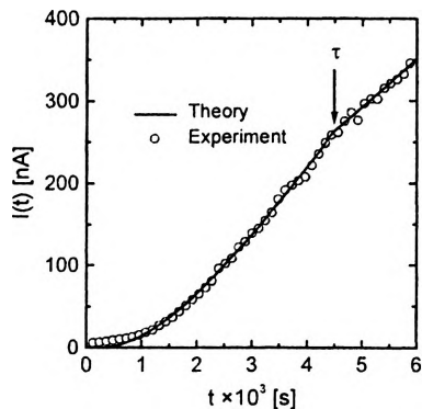
Fig. 3. Experiment – a comparison with theory. Measuring points have been obtained for T_1 = 423 K and T_2 = 353.8 K. The fitting parameters: W_a = 0.61 eV, \mu_0 = 2 cm 2 /Vs. The arrow marks the ions time-of-flight \tau = 4440 s.
