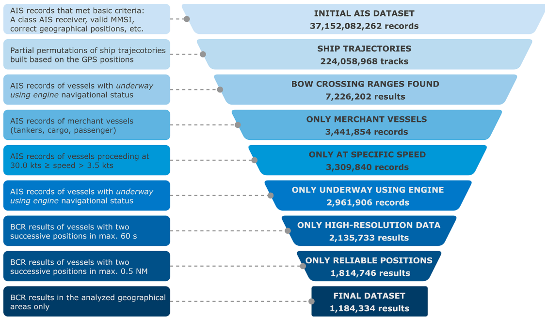
Fig. 7. Funnel chart with the major filtering steps.
