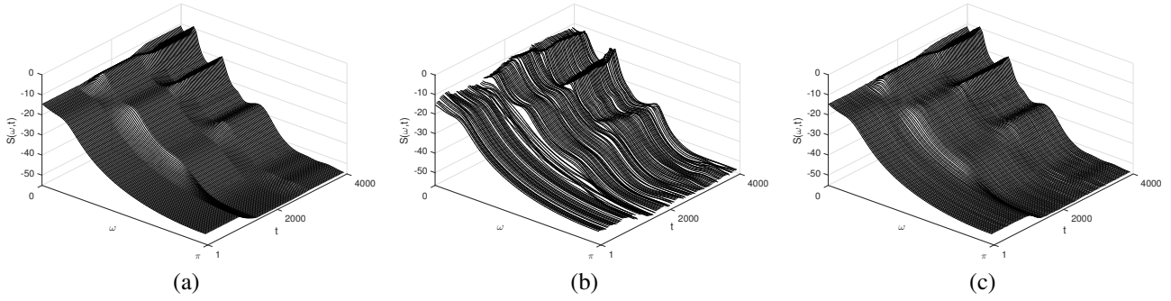
Fig. 2: True time-varying spectrum of the simulated autoregressive process (a), its E^2WLMF estimate obtained for a single process realization (b), and the plot obtained after averaging estimation results over 100 realizations (c). All plots were obtained for the left signal channel and smooth parameter variations.
