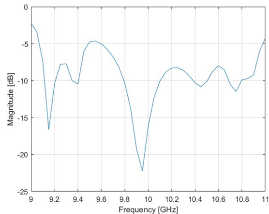
Fig. 10. Reflection coefficient of the designed antenna array
