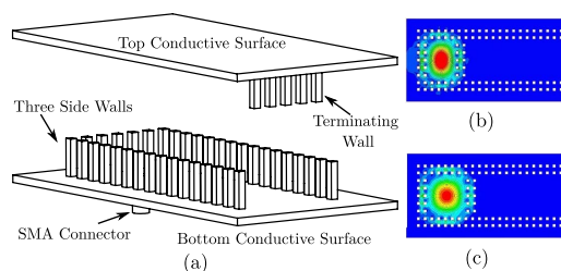
FIGURE 1. (a) An illustration of the proposed tunable GGW cavity resonator, and the electric field distributions (using eigen analysis) of the tunable resonator for two different lengths corresponding to different resonance frequencies at (b) f = 14.3 GHz and (c) f = 12.6 GHz.
