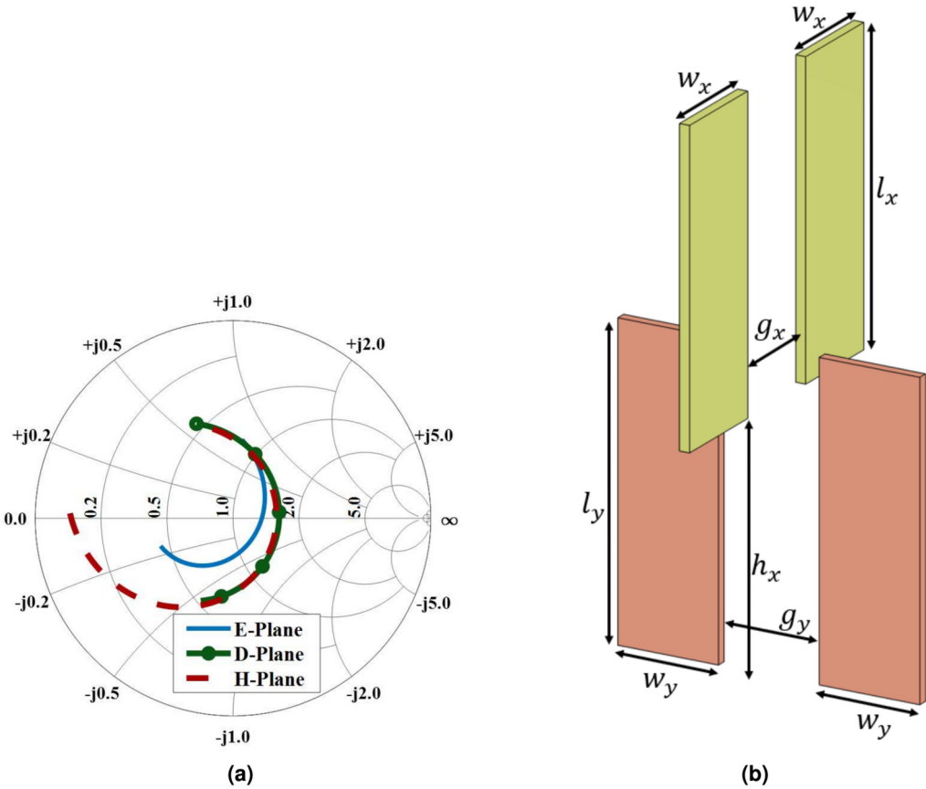
Fig. 10. (a) Smith Chart representation of array at extreme angles between 9 and 10.25 GHz. (b) Configuration to compensate the impedance mismatch.
