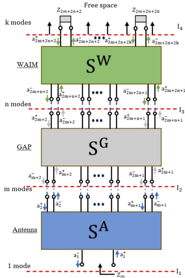
Fig. 3. Equivalent model for the loaded array formed by three cascaded GSMs.
