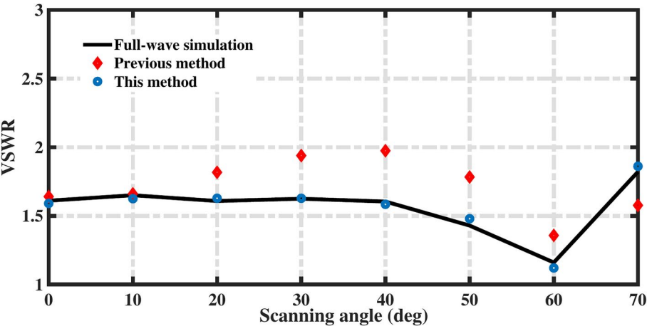
Fig. 13. Accuracy comparison of this method with previous one 22 for various scanning direction at H-plane.
