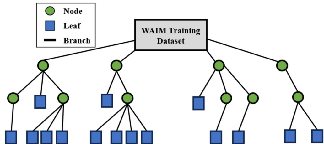
Fig. 5. Decision tree prediction structure.
