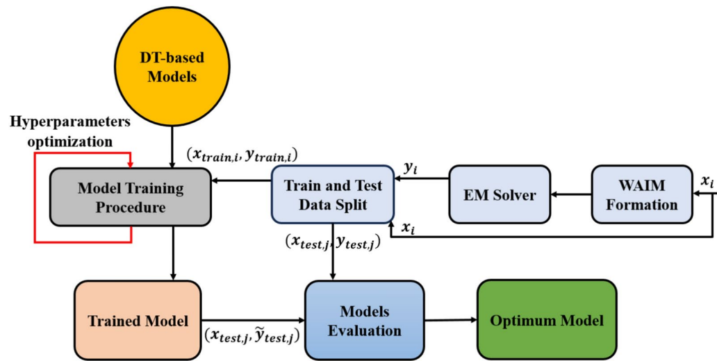
Fig. 4. Training procedure and selection of the best SM model.
