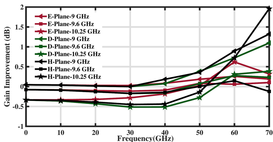
Fig. 17. Relative gain improvement of the array by adding WAIM.
