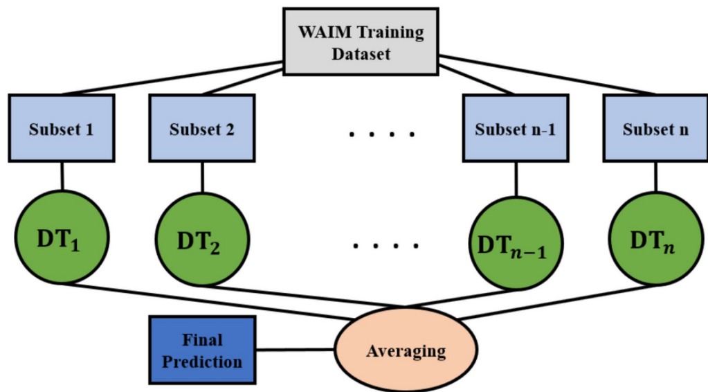
Fig. 6. Bagging method prediction structure.
