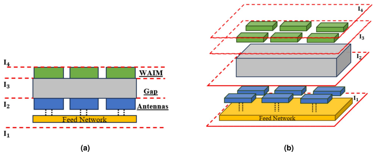
Fig. 1. (a) Example of the array with the WAIM and the gap between them. (b) Exploded view of the structure with the reference planes of each layer.
