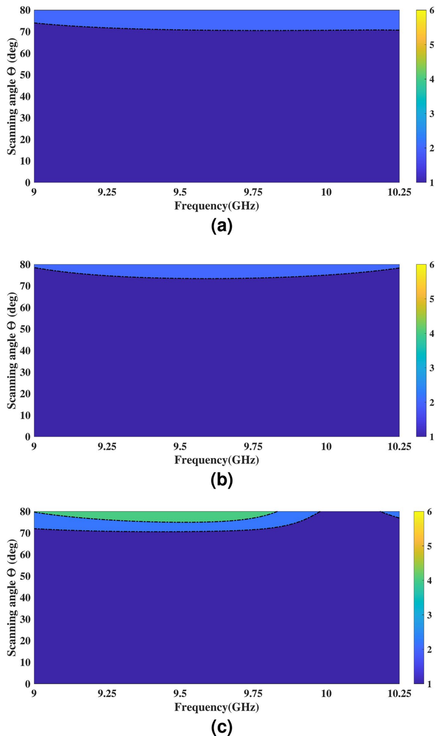
Fig. 15. VSWR results of full-wave simulation of the designed array by considering a dielectric in the intermediate layer (a) E-plane, (b) D-plane, (c) H-plane. First contour shows VSWR less than 2.
