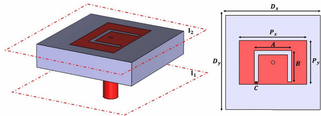
Fig. 8. Perspective and top view of the coaxial-fed U-slot.
