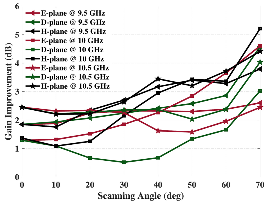
Fig. 21. Relative gain improvement of the waveguide array by adding the WAIM.
