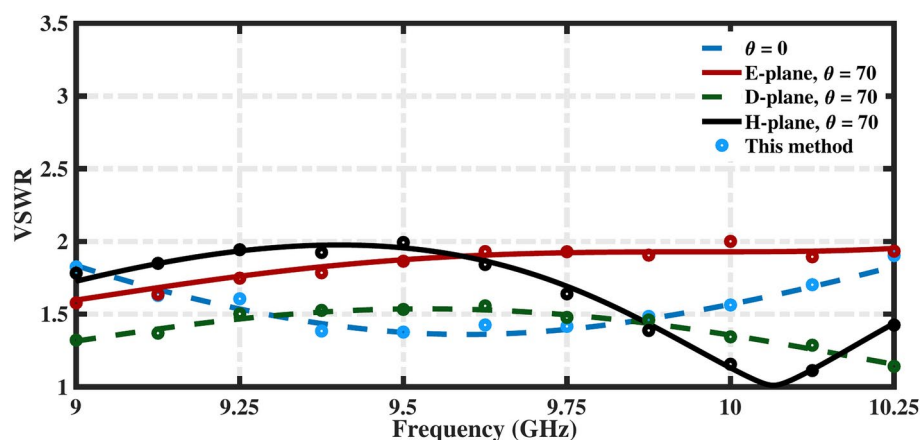
Fig. 16. Comparison between the outcome of proposed method and HFSS simulation results.
