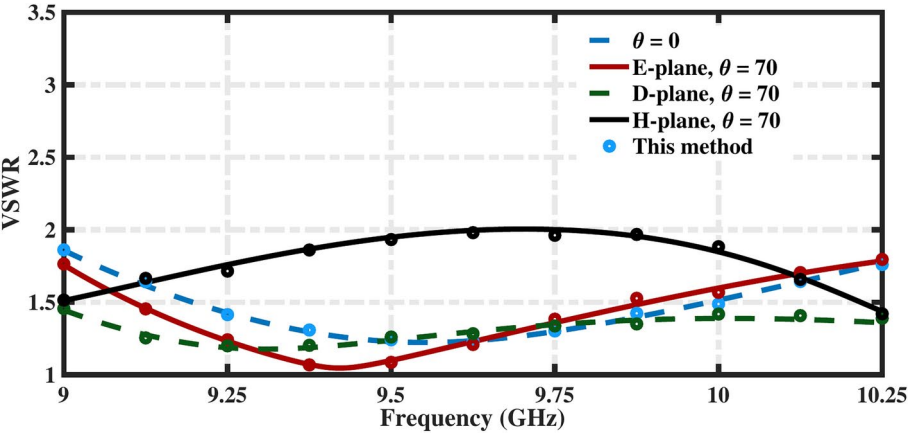
Fig. 12. Comparison between the outcome of proposed method and full-wave simulation results.
