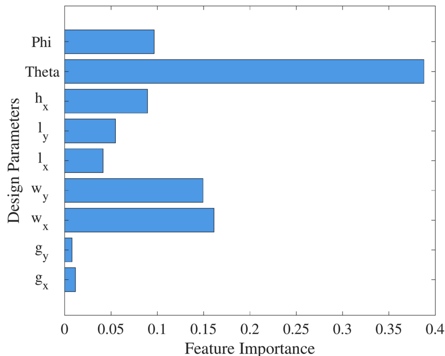
Fig. 22. Sensitivity analysis on the WAIM parameters.
