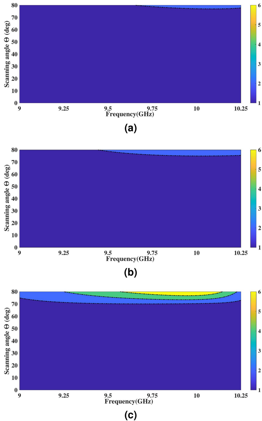
Fig. 11. VSWR of full-wave simulation of the unit cell of loaded structure as a function beam scanning direction and frequency in the desired bandwidth at (a) E-plane, (b) D-plane, (c) H-plane. First contour shows VSWR less than 2.
