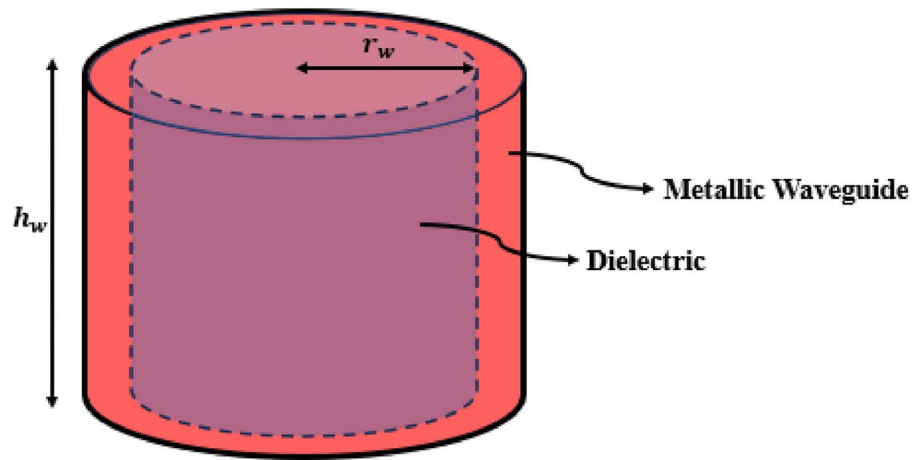
Fig. 18. Metallic waveguide filled with dielectric as the array element with r_w = 6.2 mm and h_w = 25 mm.
