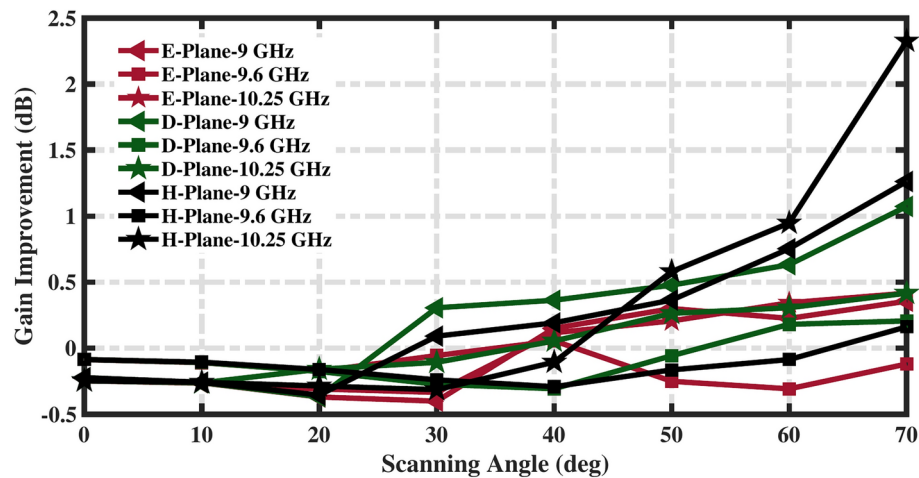
Fig. 14. Relative gain improvement of the array by adding WAIM.
