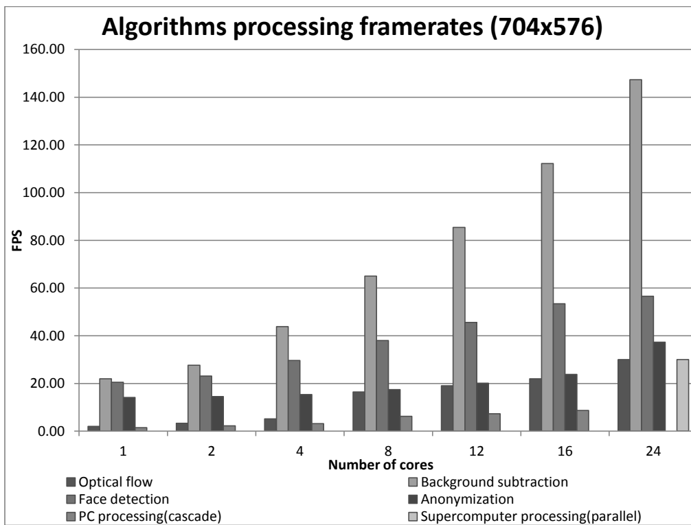
Figure 16: Algorithms processing framerates for PAL resolution data streams
