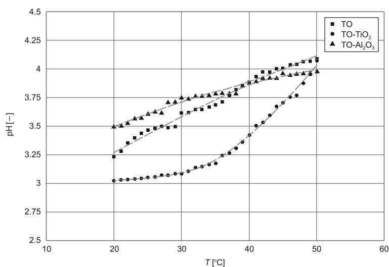
Figure 11: PH of TO- \text{Al}_2\text{O}_3 and TO- \text{TiO}_2 nanofluids with nanoparticle concentration of 0.1%.
