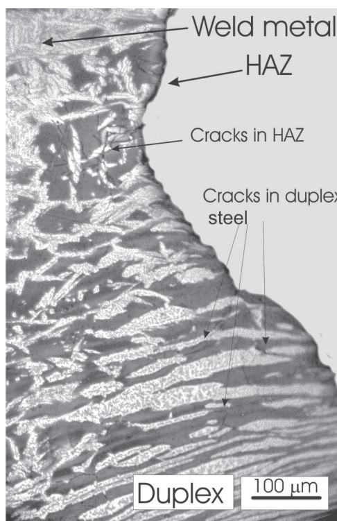
Fig. 13. Crack propagation paths at “I” welded specimen after SSR test in boiling MgCl 2 solution at 125°C
