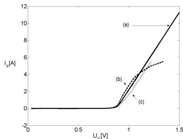
Fig. 7. The DC characteristics for one of STD12S60 diodes measured in three different systems: (a) – system No. 1, (b) – system No. 2, (c) – system No. 3.
