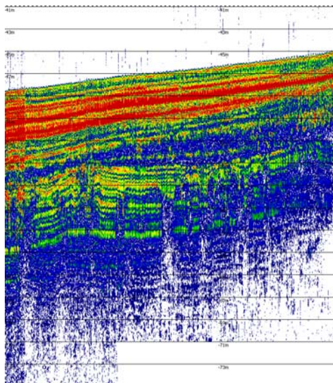
Fig.14. . Envelope from 5120 samples – 6kHz 2p
