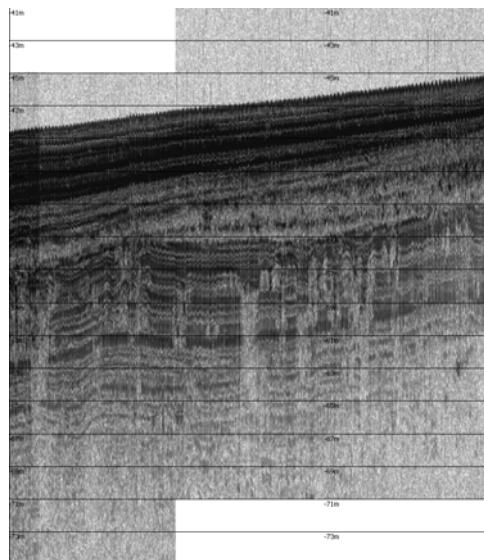
Fig.15. Envelope from 5120 samples – 6kHz 2p
